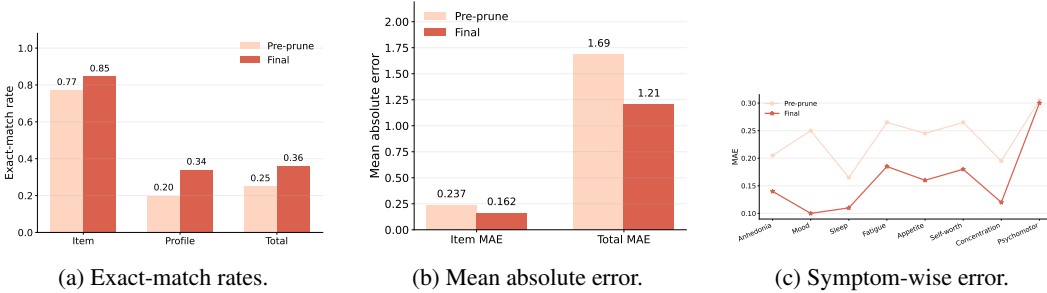
Figure 2: Comparison of how agent self-report PHQ-8 scores based on given cues before and after pruning.
