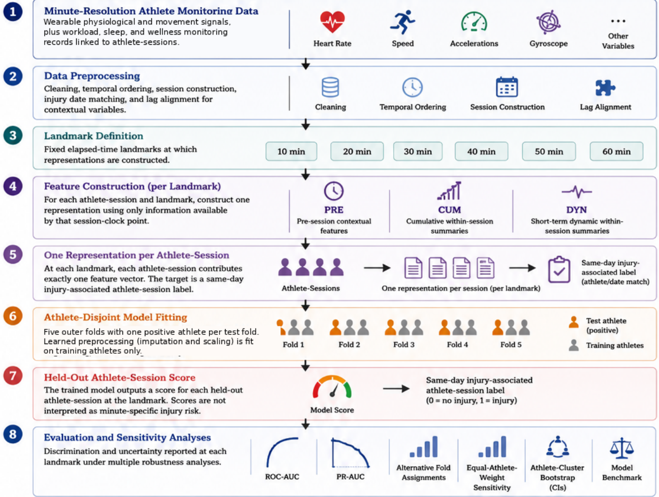
Figure 1: Overview of the landmark-based framework. At each fixed landmark, one representation is constructed per athlete-session using only information available by that session-clock point. The target remains a same-day injury-associated athlete-session label; no within-session injury-onset timestamp is assumed, and scores are not interpreted as minute-specific injury risk.
