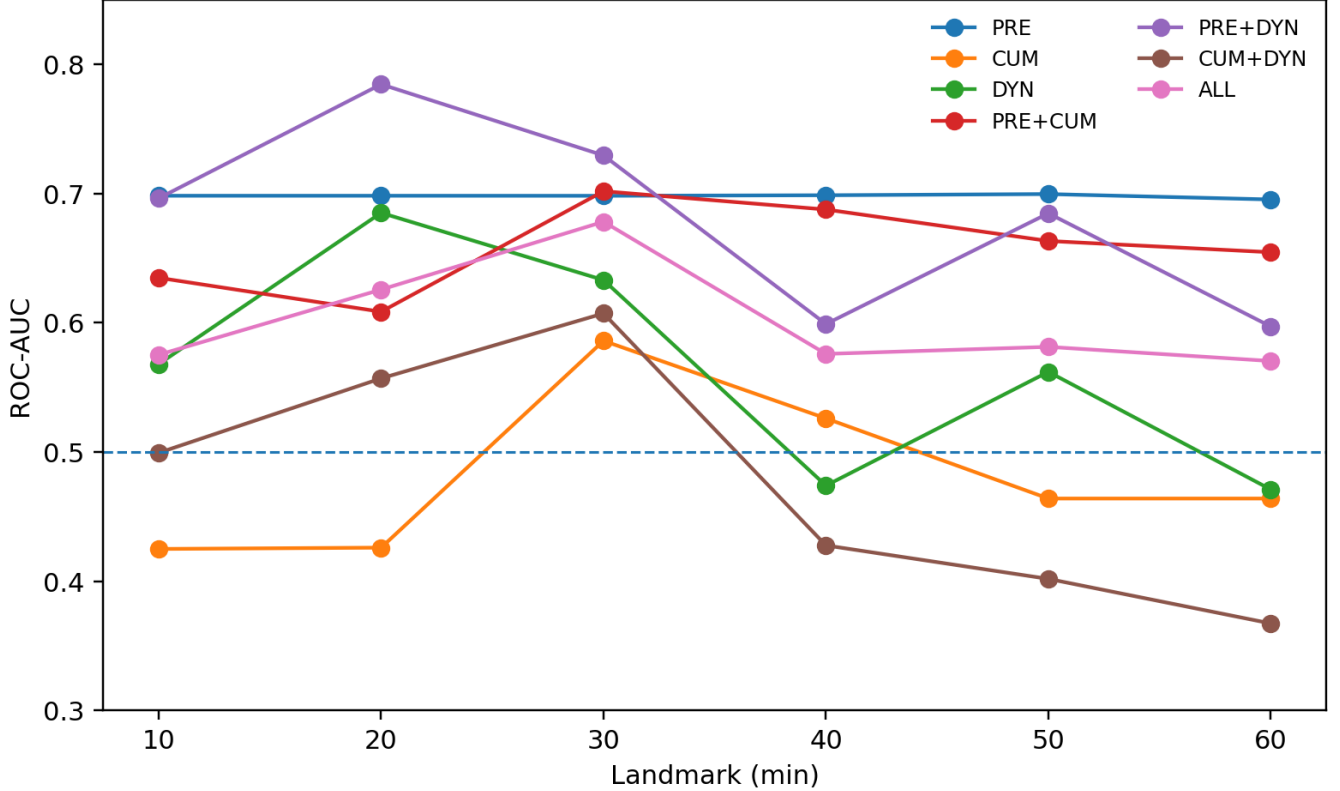
Figure 3: ROC-AUC trajectories for the seven feature-family configurations. Relative ordering changes across landmarks; no representation is interpreted as uniformly superior.
