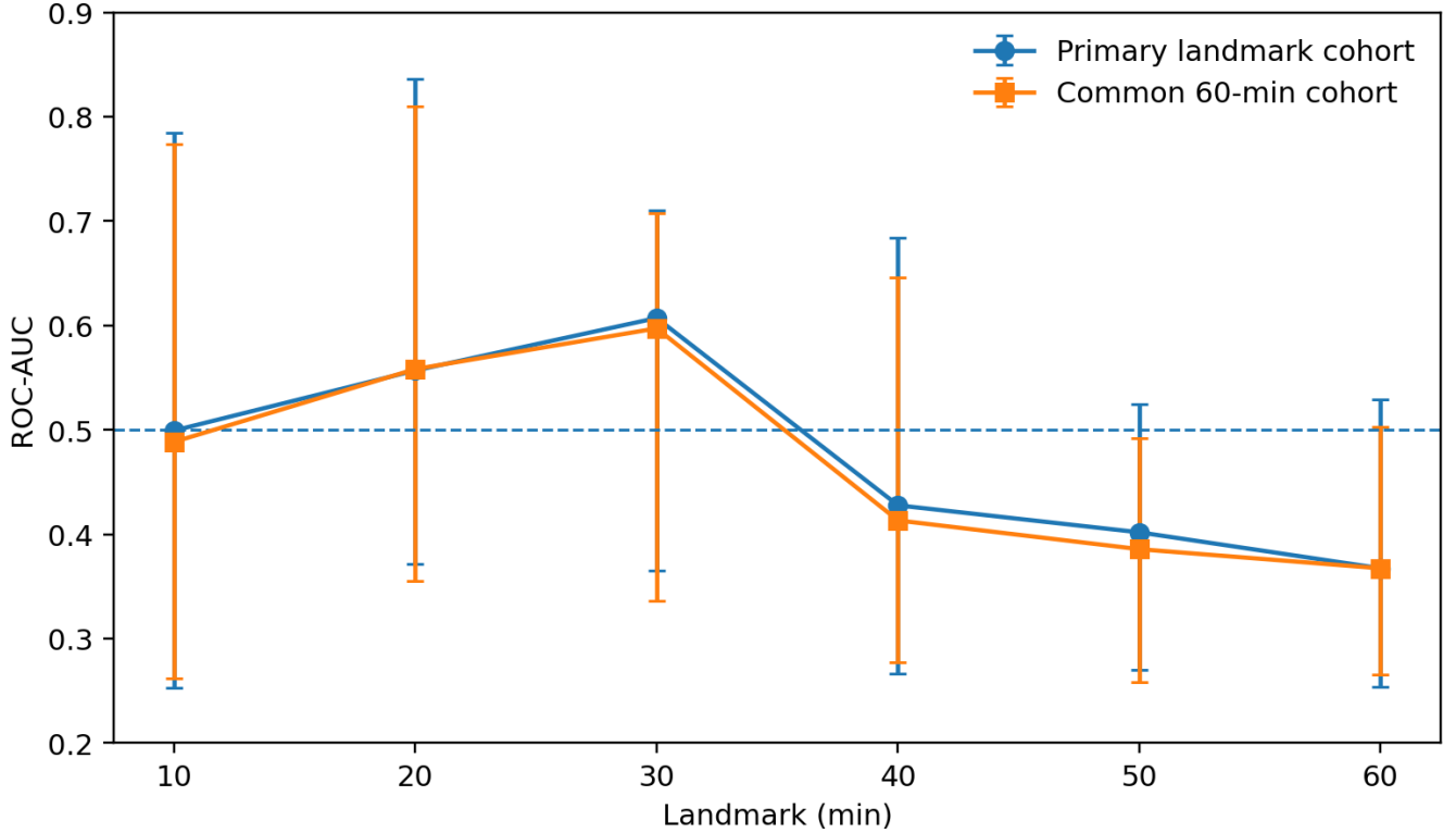
Figure 2: Primary and common-cohort ROC-AUC across landmarks. Error bars are 95% athlete-cluster bootstrap intervals; the dashed line denotes ROC-AUC = 0.5.
