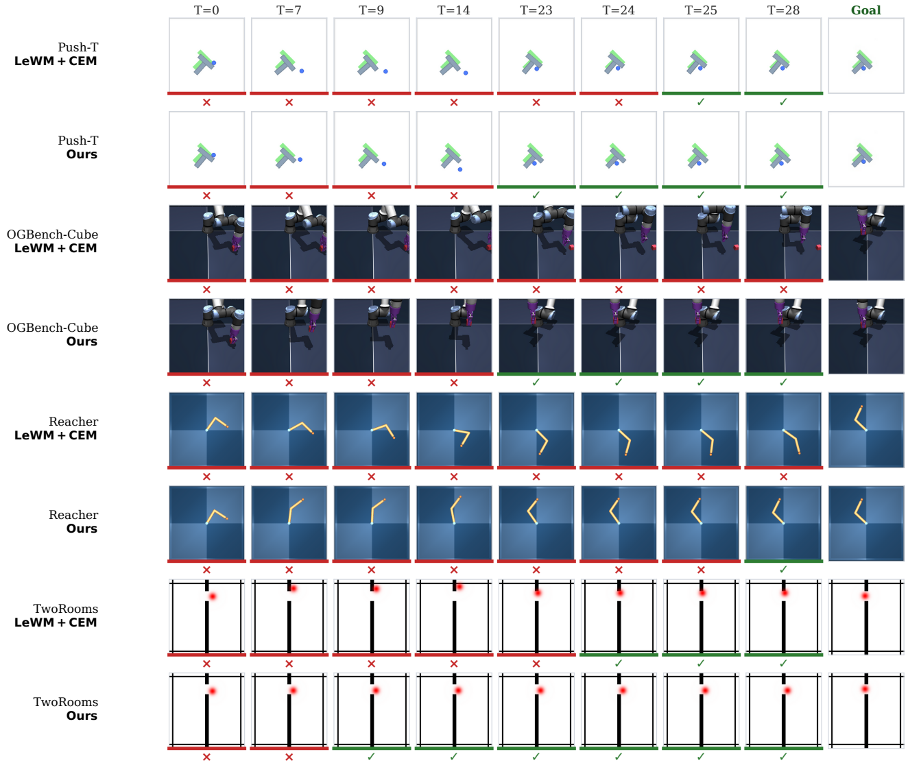
Fig. 5. Paired qualitative rollout comparison across four domains. Red crosses denote states before goal attainment, green check marks denote states at or after goal attainment, and the final column shows the goal.
