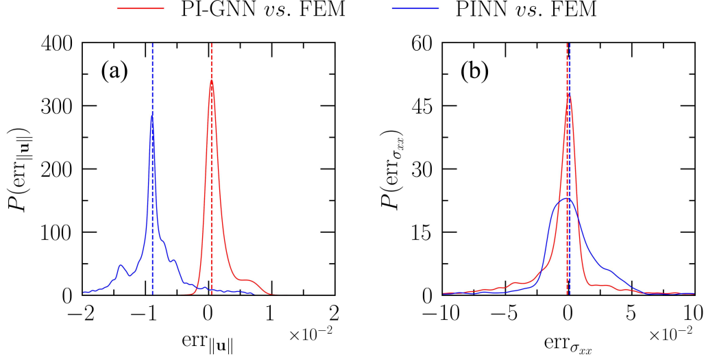
Figure 10: Spatial density of the element-wise relative error for the PINN and PI-GNN predictions against their respective FE references for the circular inclusion. (a) \text{err}_{||\mathbf{u}||} . (b) \text{err}_{\sigma_{xx}} . Nodes carrying less than 20% of the peak reference value are excluded, following Equation (23).
