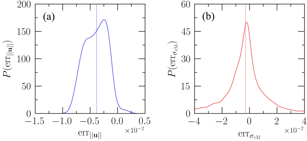
Figure 14: Relative error densities comparing PI-GNN and the FEM reference for the re-entrant inclusion. (a) Displacement magnitude. (b) von Mises Stress.
