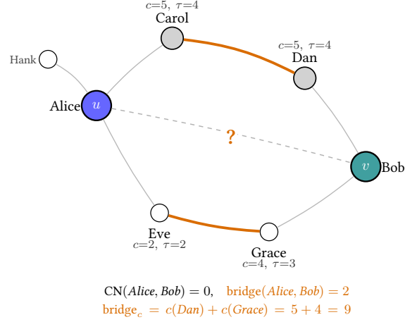
Figure 1: Running example (used throughout the paper). In a corporate email network, Alice ( u ) and Bob ( v ) have never emailed each other, so the 1-hop common-neighbour count is CN = 0 ; a cooccurrence-based structure channel sees no signal. Yet two 2-hop paths connect them: Alice–Carol–Dan and Alice–Eve–Grace, where Dan (core 5) and Grace (core 4) are Bob’s direct neighbours and Carol, Eve are the length-two intermediaries from Alice. HAWKEYE reads exactly these bridges and correctly rates Alice–Bob as a likely next-email pair. Section 3 shows this configuration is the typical informative pair on sparse temporal graphs; Section 4 explains how the cache and the slot encoder make Alice’s, Bob’s, and the intermediaries’ coreness available at query time; and §5.6 returns to this example in the case study.
