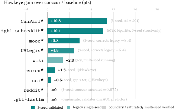
Figure 3: Per-dataset HAWKEYE swap-in gain over the DyGFormer (cooccur) baseline (test AP for DGB, test MRR for wiki); ★ = 3-seed validated (std \leq 0.011 ). Double-digit gains on CanParl (+10.8) and tgb1-subreddit (+10.1), mid single-digit on mooc (+5.8) and USLegis (+4.8), small but consistent on sparse uci/enron; on saturated reddit and degenerate tgb1-lastfm the gain correctly vanishes, tracking the training-free 2-hop discAUC predictor (§3).
