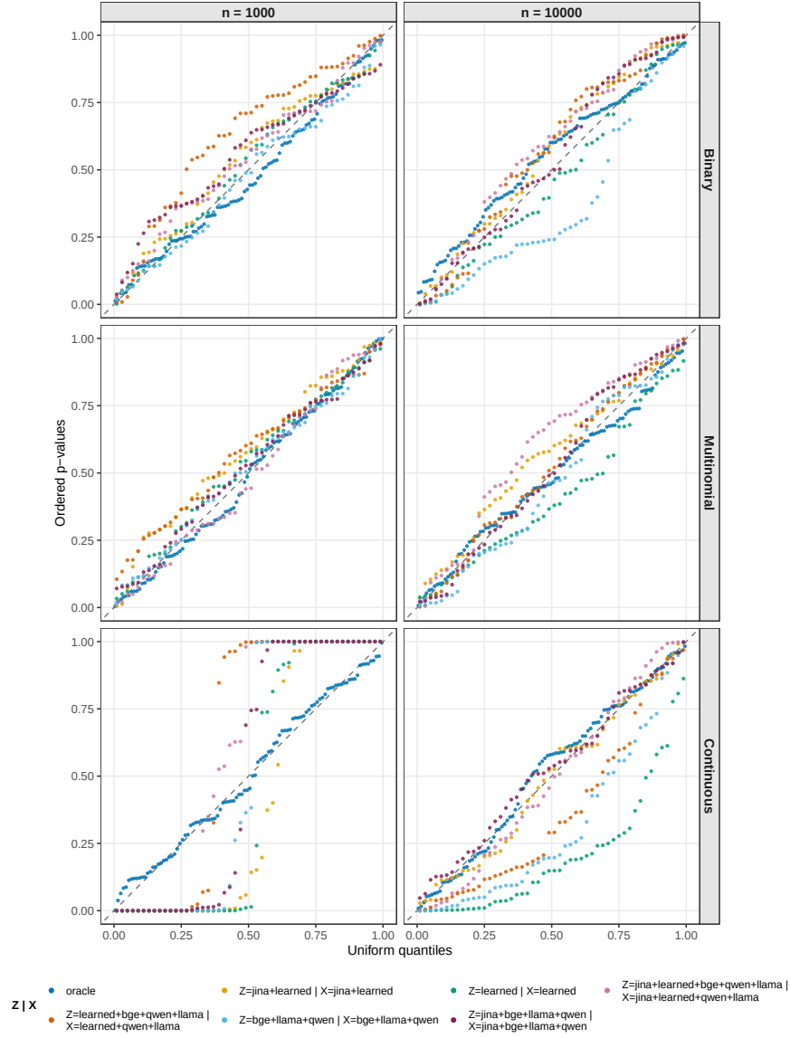
Figure 4: QQ-plots of the observed p-values against the theoretical quantiles of a uniform distribution on the interval [0, 1] for eCITs with the specified embeddings. For the PCM, the nuisance regressions on the training dataset are L_2 -penalized and those on the evaluation set unpenalized; for categorical Y the regressions of Y are multinomial logistic and those of the fitted probabilities and of \hat{f} are least squares (Appendix D.1). Y is generated under the null hypothesis from the Jina embedding Z^{\text{Jina}} at selected sample sizes (indicated in the panel titles). The diagonal black lines y = x serve as references for the theoretical quantiles of the uniform distribution on [0, 1] . If the p-values are uniformly distributed, they should align along this line.
