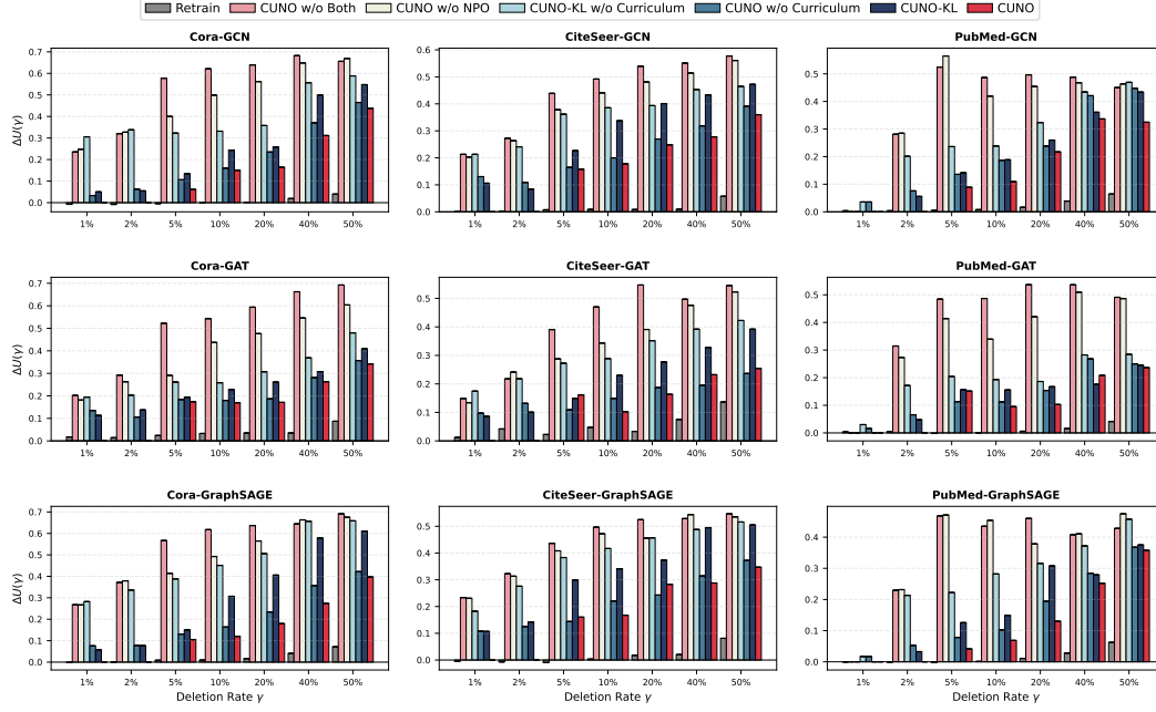
Figure 12: Full ablation study: utility drop across all dataset-GNN configurations.
