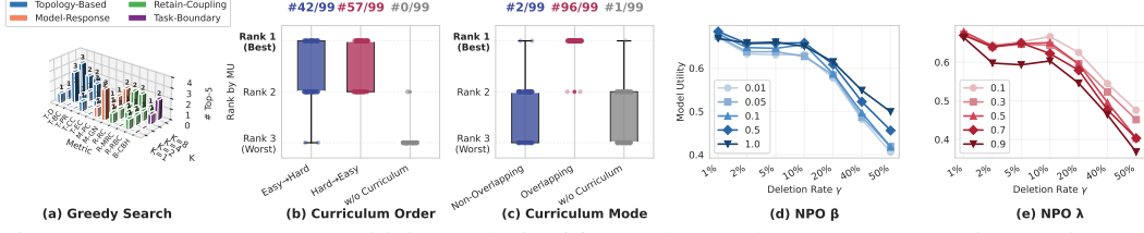
Figure 7: Hyperparameter sensitivity analysis. (a) Greedy search over 11 complexity metrics and different numbers of curriculum K : each cell counts how many of the 9 dataset–GNN scenarios a combination enters the top-5 by model utility. (b) Ranking of curriculum ordering strategies (easy-to-hard vs. hard-to-easy) under overlapping mode across 11 metrics and 9 dataset–GNN groups. (c) Ranking of curriculum partitioning modes (non-overlapping vs. overlapping). (d, e) Model utility vs. unlearn rate under varying NPO preference strength \beta and balance weight \lambda , respectively.
