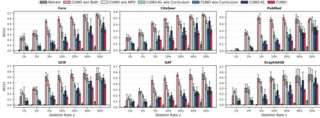
Figure 5: Catastrophic unlearning analysis across ablation variants. Compared with ablations, the full CUNO method consistently maintains the lowest utility drop across all deletion rates, confirming the complementary contributions of curriculum scheduling and NPO.
