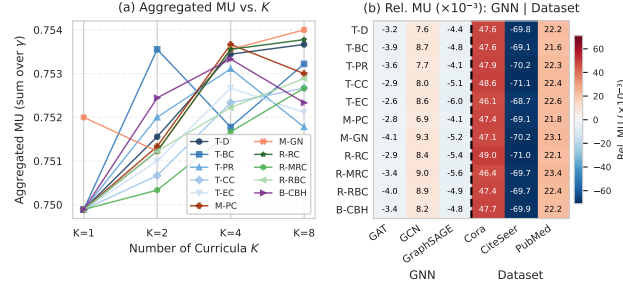
Figure 13: (a) Aggregated MU vs. K for all 11 metrics (9-scenario average); all metrics improve with K . (b) Relative MU per metric (rows) across GNN types and datasets (columns), shown as deviation from the grand mean ( \times 10^3 ). Dataset identity dominates variation (range 0.117) over GNN type (0.013).
