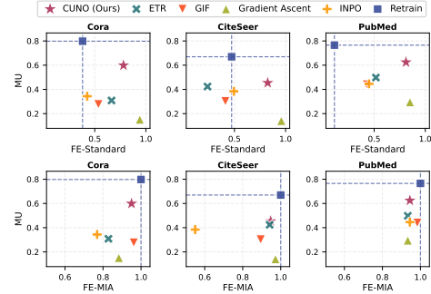
Figure 4: FE and MU at deletion rate 20%. Dashed crosshairs mark the Retrain reference. Top row (FE-Standard): a confounded metric on graphs (Retrain itself attains low FE-Standard due to neighbourhood label inference; cf. Appendix F.3); higher values alone do not unambiguously indicate better unlearning. Bottom row (FE-MIA): the calibration-transformed FE-MIA, which anchors Retrain at x=1.0 and penalises over- and under-erasing equally; the upper-right corner is the ideal calibrated position.
