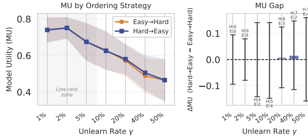
Figure 14: MU of easy-to-hard vs. hard-to-easy ordering, averaged over all 11 metrics and 9 dataset-GNN scenarios. At low deletion rates ( \gamma \leq 5\% ) the two strategies are nearly identical; at higher rates, hard-to-easy yields a growing advantage (winning 7/9 scenarios at \gamma=40\% ).
