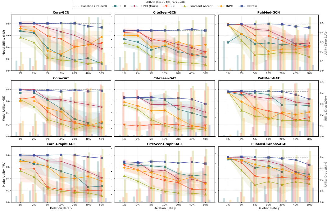
Figure 10: Full MU and utility drop \Delta U(\gamma) vs. deletion rate \gamma across all dataset-GNN configurations.
