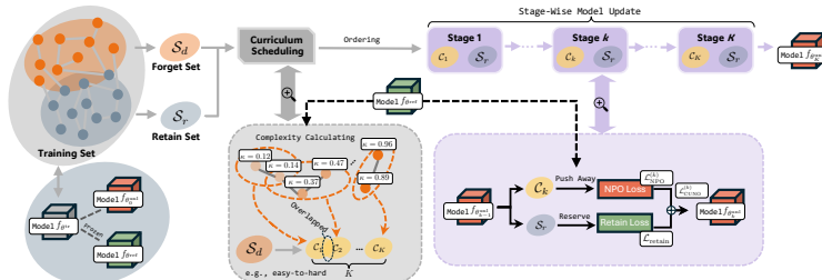
Figure 2: Schematic of CUNO. An unlearning-difficulty score orders the forget set into overlapping stages from a specific order ( when to forget ); at each stage, a distribution-level NPO objective steers the model away from a frozen reference, while a retain loss anchors utility ( how to forget ). Together they turn one-shot unlearning into a smooth, controllable progression.
