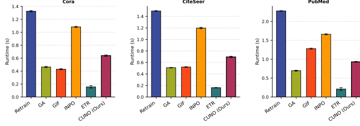
Figure 9: Runtime per method averaged over GCN, GAT, and GraphSAGE ( \gamma=20\% ). Iterative methods run to full completion; ETR and GIF are one-off procedures.
