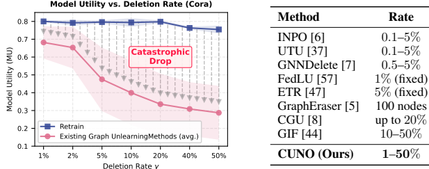
Figure 1: Left: Model utility vs. deletion rate on Cora (averaged results among existing graph unlearning methods). The gap between Retrain and existing methods grows sharply at high deletion rates ( catastrophic unlearning ). Right: Deletion rates investigated in prior graph unlearning methods. Most methods evaluate only up to 5%.
