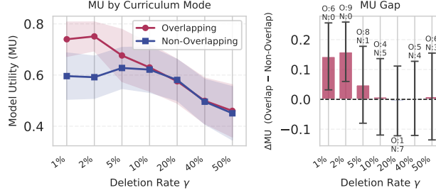
Figure 15: MU of overlapping vs. non-overlapping curriculum mode, averaged over all metrics and 9 dataset–GNN scenarios. Overlapping mode yields a large MU advantage at low deletion rates (up to \Delta\text{MU}=0.15 at \gamma=2\% ) and remains competitive across all \gamma , confirming it as the more robust default..
