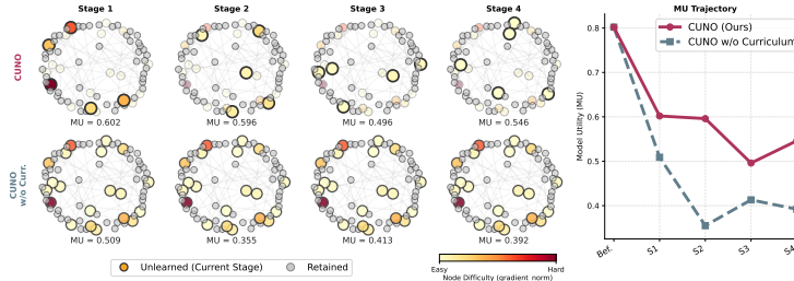
Figure 6: Qualitative comparison of CUNO and NPO-without-curriculum (Cora, GCN, gradient_norm, \gamma=50\% ). Top (CUNO): a moving spotlight advances through K=4 complexity-ordered stages. Bottom (CUNO w/o Curriculum): all forget nodes are treated uniformly with no complexity-based differentiation. Right: CUNO consistently preserves higher MU at every checkpoint.
