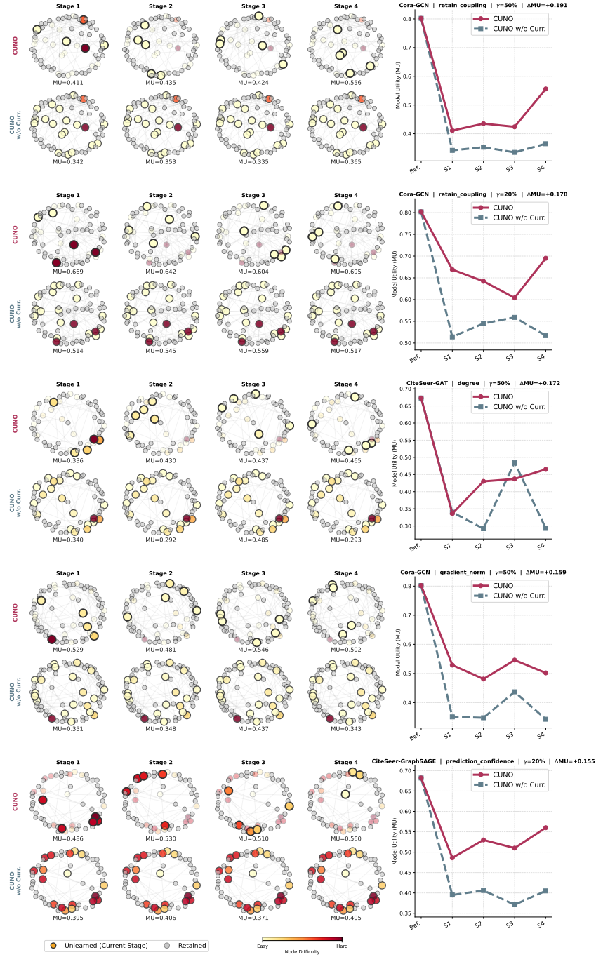
Figure 16: Additional qualitative examples (cf. Figure 6).
