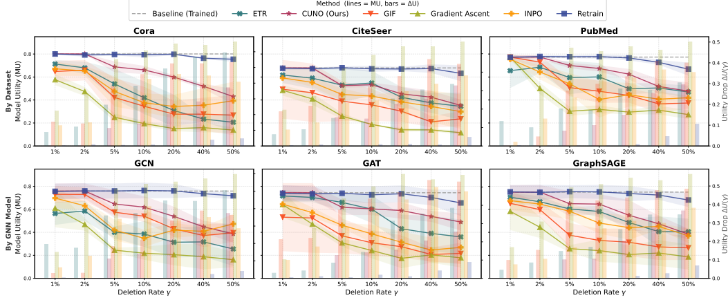
Figure 3: Model utility (MU) and utility drop \Delta U(\gamma) vs. deletion rate \gamma . Solid lines (left axis) show average MU \pm 1 std across five repetitions; bars (right axis) show \Delta U(\gamma) . Top row : results grouped by dataset, averaged over three GNN architectures. Bottom row : results grouped by GNN model, averaged over three datasets. CUNO consistently achieves lower utility drop across all cases.
