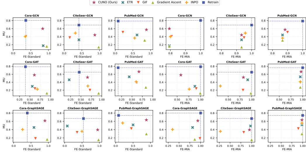
Figure 11: Full FE vs. MU across all dataset-GNN configurations ( \gamma = 20\% ).
