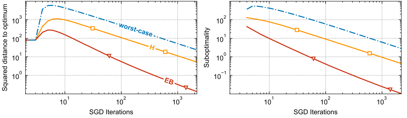
Figure 6: SGD on the covertype.binary dataset in a true single-pass regime, with b = 256 . Each panel shows the worst-case bound (dash-dotted blue line), H (solid orange line with squares), and EB (solid red line with triangles).
