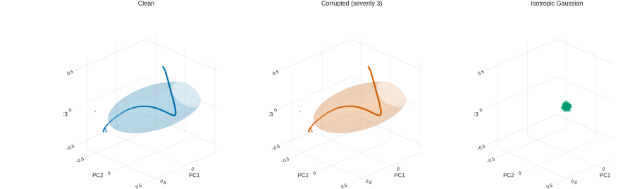
Figure 11: What the geometry diagnostic sees in the four CL configurations. Rows identify the models; columns show clean text, reversible corruption at level 3, and an isotropic Gaussian reference. Each point is one averaged text vector; true target lengths are supplied. The same clean PCA axes and scale apply across a row. CL-GP/GT spread most variance beyond the three displayed axes, whereas CL-LP/LT concentrate it in this subspace. Compare these clouds with retrieval in Figure 2, rather than reading a compact cloud as evidence of content preservation. Axes are fitted to 4,096 clean examples; each cloud displays 1,200 points. Surfaces span two standard deviations, not confidence regions.
