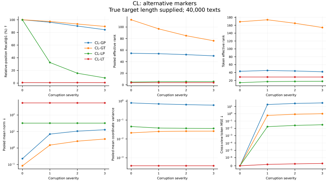
Figure 23: Full-cohort CL heldout diagnostics across severity, using oracle length. Retrieval, pooled and token effective rank, mean magnitude, variance scale, and cross-view error are shown separately. The bottom row uses a symmetric logarithmic scale with a linear region near zero. These curves use the original 40,000-item numeric summaries, independently of the smaller visualization subset.
