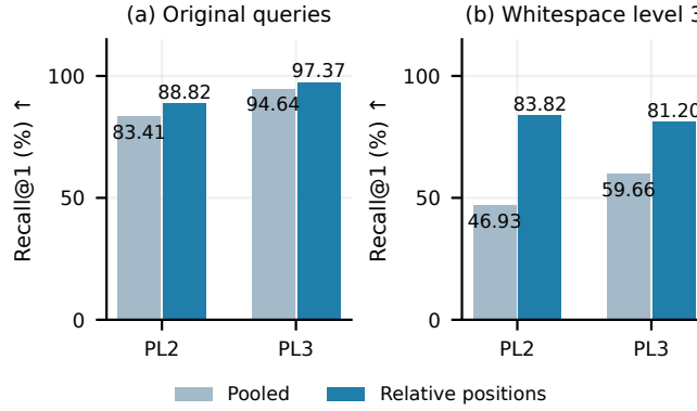
Figure 9: Position improves access within a fixed checkpoint and predicted length. Gray pools states; blue compares 16 relative positions. All 1,941 changed-input queries search the same 1,954 targets. At maximum whitespace perturbation, PL2/PL3 gain 36.89/21.54 points.
