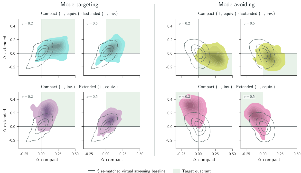
Figure 4: Density plots showing the difference in shape Tanimoto scores compared to a size-matched baseline on mode targeting and mode avoiding tasks. + and - correspond to mode targeting and mode avoiding conditioning, respectively, and equiv. and inv. correspond to using equivariant and invariant conditioning signals.
