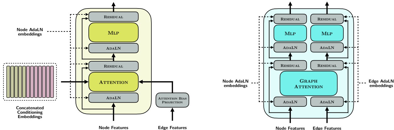
Figure 8: A transformer layer (left) and graph transformer layer (right), as used in the generator.
