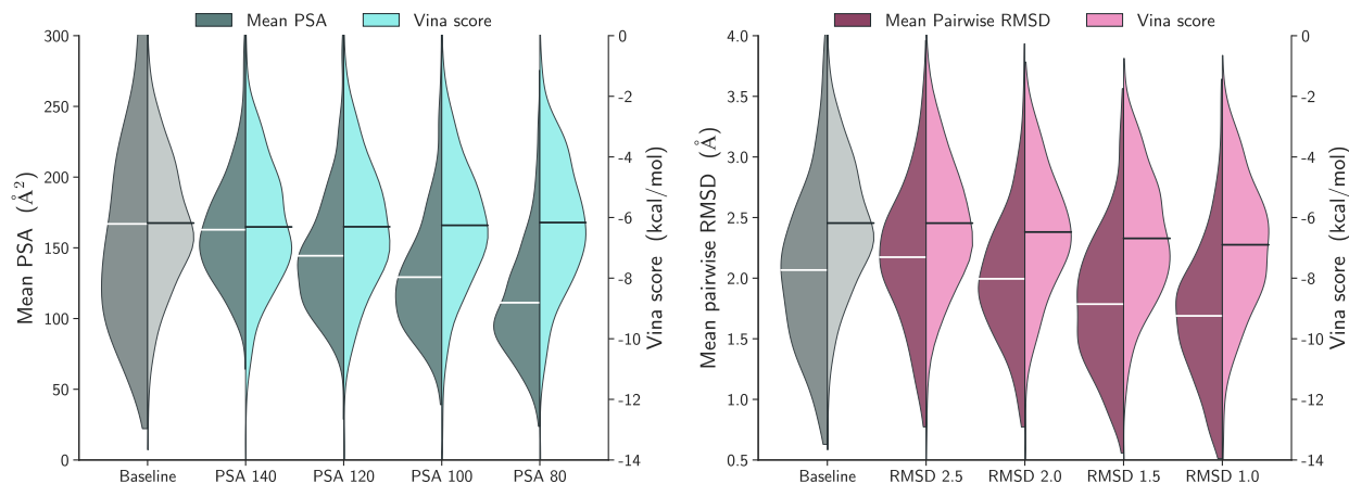
Figure 5: Distribution plots for molecular properties generated from the ensemble property optimisation benchmark. Baseline : pocket and pharmacophore conditioning; other plots come from sampling with the same condition as well as a property condition. Centre lines denote the mean of the distributions.
