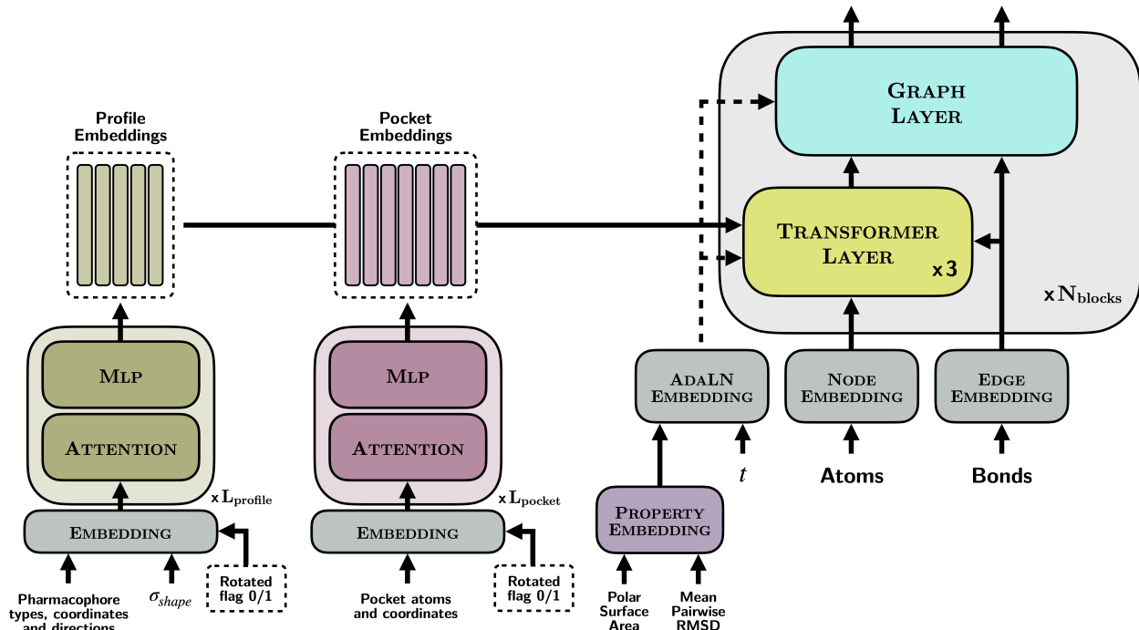
Figure 2: Our model follows an encoder-decoder design, with separate encoders for shape/pharmacophore profiles and protein pockets, as well as an ensemble property embedding module. Profile and pocket encoders also make use of adaptive layer normalisation (not shown for brevity). Encoders follow a standard transformer design, while the decoder mixes transformer with graph transformer layers, along with adaptive layer normalisation conditioning for incorporating property conditions and the flow-matching time t .
