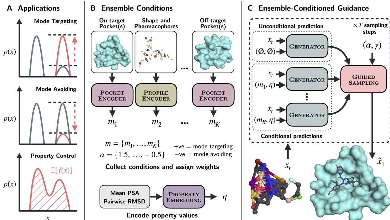
Figure 1: Overview of the ensemble-conditioned guidance framework. A: Use-cases of our framework visualised in terms of how they can be used to optimise modes and properties of the conformational ensemble. B: Conditioning signals supported by our model; modes can be represented by shapes, pharmacophore profiles or protein pockets, and properties are target scalar values. Conditioning weights \{\alpha_1, \dots, \alpha_K\} are assigned to each mode condition, m_i . In practice, conditions which share a reference frame can be grouped into a single m_i . C: Guided sampling with ensemble conditions, where x_t refers to the partially denoised molecule, and \gamma is the strength of conditioning, analogous to classifier-free guidance.
