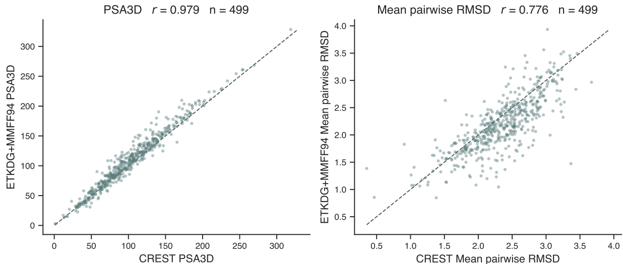
Figure 9: Scatter plots comparing mean PSA (left) and mean pairwise RMSD (right) for ensembles computed using CREST (x-axis) and our fast ensemble approximation approach (y-axis).
