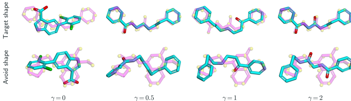
Figure 3: Generating molecules to target an extended shape while avoiding a compact shape for different conditioning strengths, \gamma , where \gamma = 0 refers to unconditional generation. The two reference molecules are shown in magenta, while yellow points show the shape profiles used for conditioning. The conformer with the highest Gaussian shape overlap to the reference is plotted, and \sigma_{shape} = 0.2 was used in all cases.
