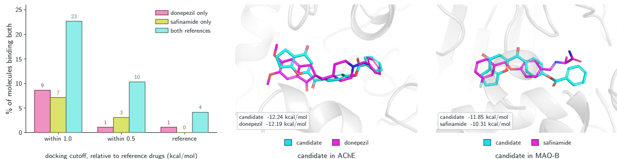
Figure 6: Dual-target binder design for AChE and MAO-B. Left: the proportion of generated molecules which bind both pockets, at cutoffs set relative to the two reference drugs’ own docking scores (AChE -12.19 , MAO-B -10.31 kcal/mol), when conditioning on donepezil only, safinamide only, and both references. Centre and right: the best joint candidate in its docked pose (cyan) overlaid on the crystal pose (magenta) of donepezil in AChE and of safinamide in MAO-B. Scores are from docking both the candidate and the reference drug into each pocket.
