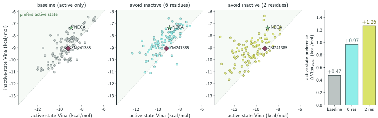
Figure 7: Active-state-biased design for the A2A adenosine receptor. Left three panels: every generated molecule placed by its docking score against the active and inactive receptor, where points above the diagonal prefer the active state, shown for the active-pocket-only baseline and for the two CoM shift thresholds used to build the inactive-pocket negative. NECA (agonist) and ZM241385 (antagonist) are docked through the same pipeline as reference points. Right: mean \Delta V_{\text{ina}}^{\text{state}} for each run.
