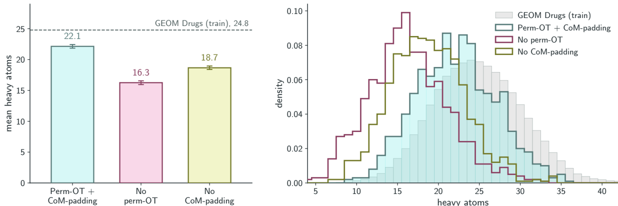
Figure 10: Unconditional size distributions for the three training setups, all trained on GEOM Drugs without the pocket encoder. Left: mean generated size, with the GEOM Drugs training mean marked. Right: full generated size distributions against the training distribution. Sizes are taken from the model’s pad token predictions. Error bars are 95% percentile bootstrap intervals over 2000 resamples of the 1000 molecules generated per model.
