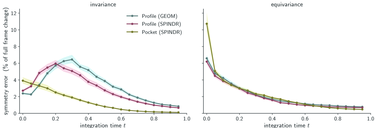
Figure 11: Symmetry error against integration time, for the profile encoder on GEOM Drugs and SPINDR ligands and for the pocket encoder on SPINDR pockets. Left: invariance, where the condition is rotated and the prediction should not move. Right: equivariance, where the state and condition are rotated together and the prediction should rotate with them. Errors are given as a percentage of the distance the prediction would have moved had it broken the symmetry instead, which ranges from 2.6 to 5.0 Å over the encoders and snapshots shown. Bands are 95% bootstrap intervals over 64 systems, each averaged over 8 rotations.
