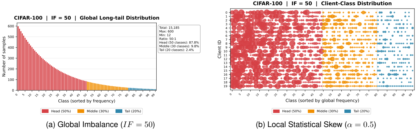
Fig. 2: Visualization of the proposed Double Heterogeneity under the rigorous Scenario C configuration (using CIFAR-100 at IF = 50 and \alpha = 0.5 as a representative prototype). (a) Global Imbalance: The aggregated global distribution exhibits a steep exponential decay, severely starving the Tail classes. (b) Local Statistical Skew: The bubble chart illustrates the extreme non-IID data partition across 20 simulated edge clients. The severe fragmentation and extensive blank regions in the right hemisphere visually demonstrate that tail categories are completely absent across the vast majority of local clients.
