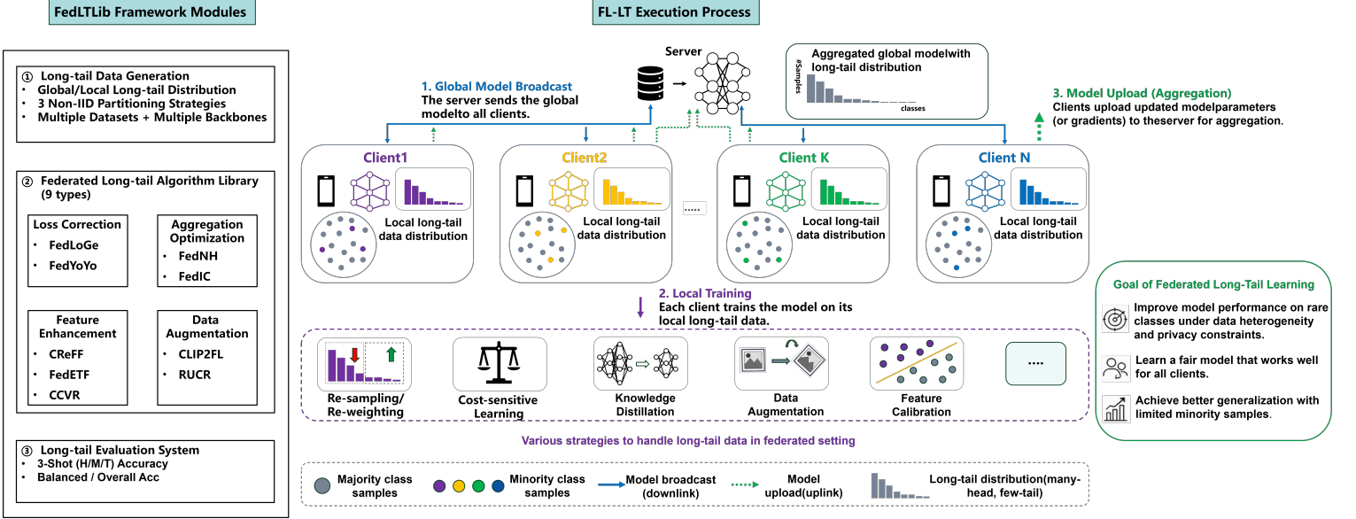
Fig. 1: The overall architecture of the FedLTLib framework, consisting of the FedLTLib Framework Modules (left) and the FL-LT Execution Process (right). The framework provides a standardized project structure for data synthesis, server-side orchestration, and client-side training. The execution process illustrates the “Double Heterogeneity” challenge across distinct clients and summarizes mainstream optimization paradigms integrated into our benchmark, specifically Cost-sensitive Learning, Knowledge Distillation, and Feature Calibration, to achieve global fairness and tail-class generalization.
