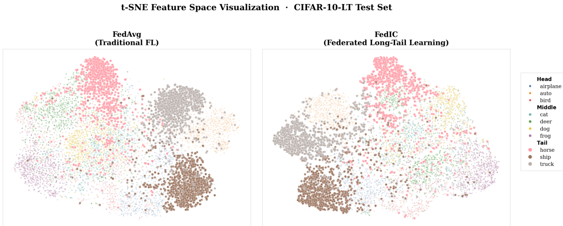
Fig. 4: t-SNE visualization of the global model's feature space on the CIFAR-10-LT test set. (Left) Traditional FL (FedAvg) exhibits severe feature entanglement, where tail classes, such as horse, ship, and truck, collapse into the feature clusters of majority classes. (Right) FedIC maintains highly structured representations with clear decision boundaries, effectively preventing minority classes from being absorbed by the head classes.
