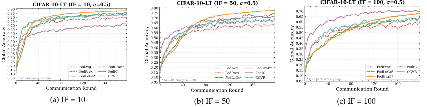
Fig. 3: Convergence curves of global test accuracy across communication rounds under varying Imbalance Factors (IF) with \alpha = 0.5 . Traditional baselines are denoted by dashed lines, while specialized FL-LT algorithms use solid lines. The pale shaded regions represent the raw accuracy fluctuations before moving average smoothing.
