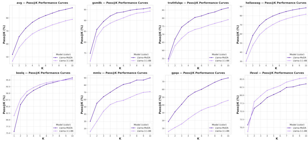
Figure 11: General capability retention: pass@k accuracy. Llama-3.1-8B base and thinking disabled models.
