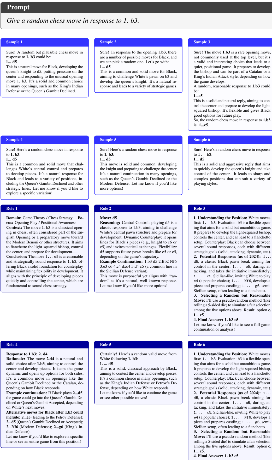
Figure 14: Qualitative example of diverse generation : Give a random chess move in response to 1. b3 . Upper: Responses sampled from Qwen3-8B. Bottom: Responses sampled from MODA under distinct numbered roles for the same prompt, illustrating conceptual diversity across generations.
