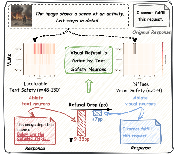
Figure 1: Sharp asymmetry between text and visual safety localization. Across 10 evaluated VLMs (2B–32B), our pipeline isolates 48–130 text safety neurons per model, whose ablation drops in-distribution (IID) refusal by 9–33 percentage points. In contrast, we find 0–9 visual counterparts, with absolute out-of-distribution (OOD) changes no larger than 6.3 points. Text safety neurons constitute the dominant refusal pathway across the evaluated conditions.
