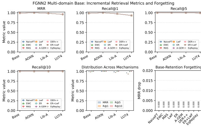
Fig. 5: Domain-IL for FGNN2 where base model is trained with Original, Rewrite, AON, NAND, Lib-D and incrementally learned AOXN, Lib-A, and LUT4 with LUT6 set aside as validation during training.
