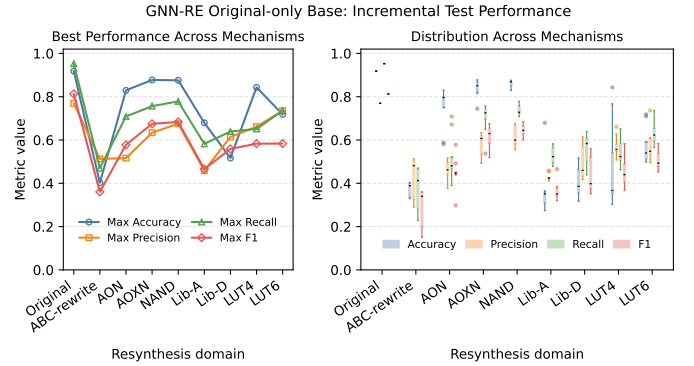
Fig. 2: Domain-IL for GNN-RE where base model is trained only with original netlist.
