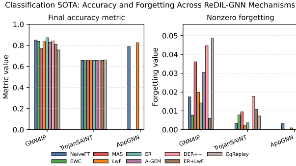
Fig. 4: Domain-IL performance for GNN4IP, TrojanSAINT, and AppGNN where training setup is same as Fig. 3.
