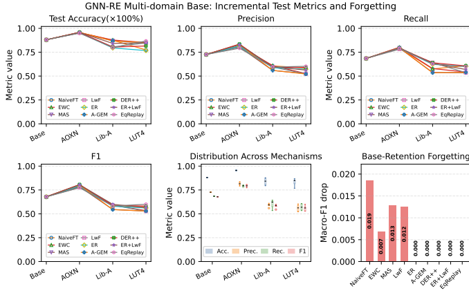
Fig. 3: Domain-IL for GNN-RE where base model is trained with Original, Rewrite, AON, NAND, Lib-D and incrementally learned AOXN, Lib-A, and LUT4 with LUT6 set aside as validation during training.
