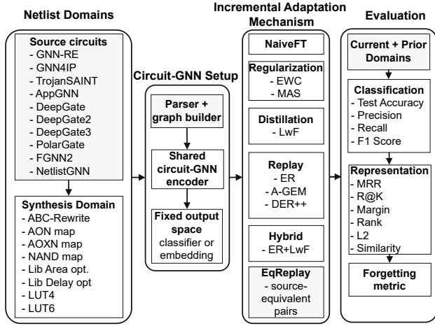
Fig. 1: High-level ReDIL-GNN methodology. Source circuits are converted into multiple resynthesis-domain views and parsed into circuit graphs. A shared circuit-GNN encoder with a fixed classifier or embedding space is then adapted through different incremental learning mechanisms. Evaluation is performed on both current and prior domains, using classification metrics for task-specific models, retrieval metrics for representation-learning models, and forgetting metrics to quantify retention.
