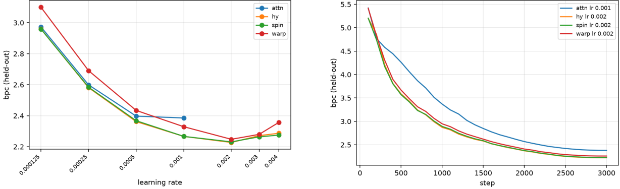
Figure 2: Repository corpus, window 256: learning-rate grid (left) and held-out curves at each schedule’s best rate (right).
