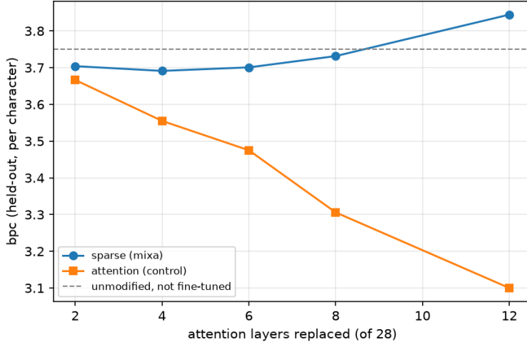
Figure 3: Replacing k of 28 attention layers in Qwen3-0.6B. The sparse variant is flat; the attention control keeps improving as it is given more layers to fine-tune.
