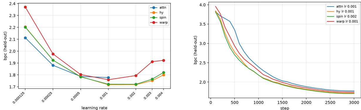
Figure 1: Public corpus, window 256: learning-rate grid (left) and held-out curves at each schedule’s best rate (right).
