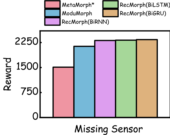
Fig. 15. FT performance under single-limb observation dropout
