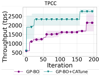
Figure 6: Performance of CATUNE integrated with GP-BO under knowledge-guided suggested ranges.
