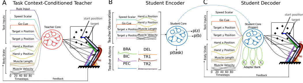
Figure 2: Teacher-student framework for learning motor adapters (A) Task context-conditioned teacher . A recurrent network controls a two-link, six-muscle biomechanical arm in closed loop [18]. (B) Student encoder . A shared LSTM core network reads the teacher’s full demonstration (observations and muscle commands, but not the rule input) and segments each trajectory into three output probabilities: what task is being done p(task) , distribution p(z) over K = 10 latent codes, and a distribution p(b) of the boundary between the two task segments. (C) Student decoder . The same core network rolls out in closed loop with only body-state feedback and task inputs (no teacher actions). The encoder-sampled code activates the corresponding adapter, which perturbs the cortical hidden state at each timestep.
