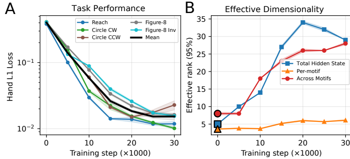
Figure 4: Emergent low-rank structure in the adapter bank. (A) Held-out hand L_1 per task and mean over training. (B) Effective rank (95% variance) of three quantities computed from closed-loop rollouts: the recurrent core’s hidden-state manifold, the per-adapter perturbation subspace (averaged across adapters), and the union of all adapter perturbations. Shaded bands are bootstrap standard errors.
