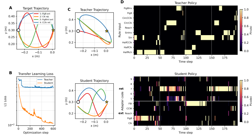
Figure 7: Compositional transfer to a butterfly trajectory. A second out-of-distribution test using a four-segment butterfly composed of (Figure-8 extension, Clockwise retraction, Figure-8 Inverse extension, Counter-clockwise retraction); none of these pairings appeared in either network’s training data. (A) The butterfly target trajectory, with each 50-timestep segment shown in a separate color. Open circle marks the home position; star marks the reach target. (B) Hand L_1 during transfer optimization. Both networks are frozen and a 10-dimensional soft policy over the network’s task interface is optimized for 600 steps. The student reaches hand L_1 \approx 0.011 , while the teacher plateaus at \approx 0.058 , a \sim 5\times gap. (C) Final teacher (top) and student (bottom) hand trajectories. The student recovers the butterfly’s figure-8-like crossing structure; the teacher’s trajectory is qualitatively distorted. (D) Final policies. Top: teacher rule-input weights over time. Bottom: student adapter-code weights.
