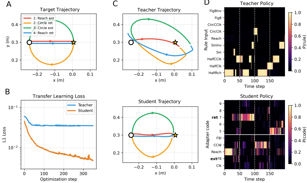
Figure 6: Out-of-distribution compositional transfer. (A) The two-petal target trajectory, composed of four movement segments stitched together in a novel combination. (B) Hand L_1 during transfer optimization, in which both networks are frozen and a 10-dimensional soft policy over the network’s task interface is optimized for 350 steps via gradient descent. Final teacher L_1 \approx 0.04 ; final student L_1 \approx 0.005 . (C) Final teacher (top) and student (bottom) hand trajectories under the optimized policies. Open circle marks the home position; star marks the reach target. (D) Final policies. Top: teacher rule-input weights over time. Bottom: student adapter-code weights.
