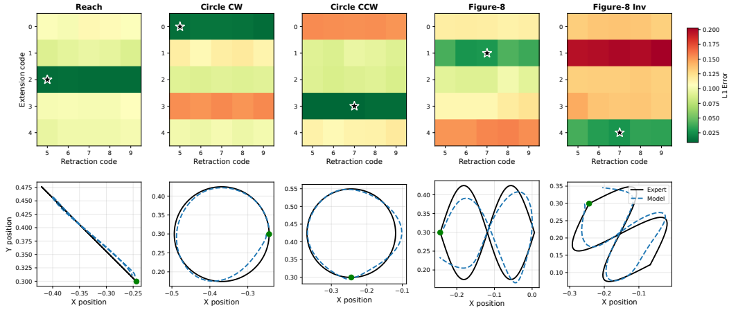
Figure 3: Student execution of compound movements. Top row: Hand-trajectory L_1 error of the trained student under all 25 forced (extension code, retraction code) pairs, for each of the five compound tasks. Rows index the five extension codes ( z_0 – z_4 ); columns index the five retraction codes ( z_5 – z_9 ). Stars mark the natural code pair selected by the encoder. Bottom row: Expert (black) and student (blue, dashed) hand trajectories under the encoder’s natural code choice. Green dots mark the start position.
