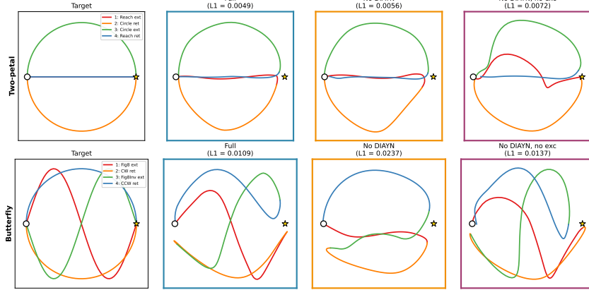
Figure 8: Ablation of auxiliary supervision components across two OOD trajectories. We test whether the architectural transfer advantage depends on the two auxiliary losses ( \mathcal{L}_{\text{DIAYN}} and \mathcal{L}_{\text{exc}} ) by training two ablated configurations: one with \beta_{\text{DIAYN}} = 0 (No DIAYN), and one with both \beta_{\text{DIAYN}} = 0 and \lambda_{\text{exc}} = 0 (No DIAYN, no exc). All other architectural choices, hyperparameters, and training details are unchanged. Final transfer trajectories on the two-petal (top) and butterfly (bottom) OOD tasks across the target and three configurations. The full configuration achieves numerically the best transfer hand L_1 on both OOD trajectories (two-petal: 0.005; butterfly: 0.011), and all three configurations achieve transfer well below the teacher baseline (two-petal: 0.04, butterfly: 0.058). The architectural advantage over the teacher therefore does not depend on the auxiliary supervisions, though auxiliary supervisions provide modest refinement to transfer accuracy.
