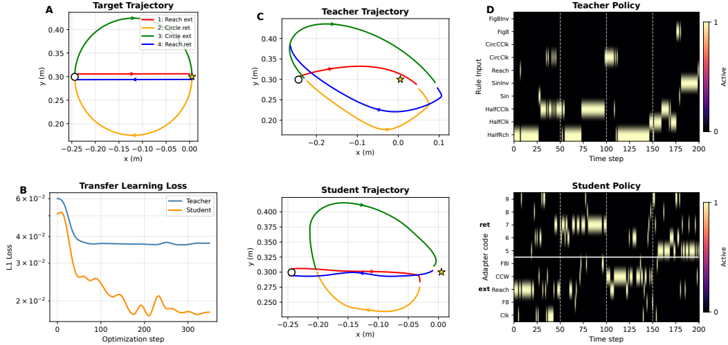
Figure 10: Compositional transfer under hard discrete policy execution. A complementary version of the two-petal transfer experiment in Figure 6, in which both networks are constrained to use hard one-hot selection over their respective task interfaces at every timestep. Optimization uses a straight-through estimator: the forward pass takes the argmax of the policy logits at each timestep (genuinely discrete selection), while gradients flow through the soft softmax distribution during backpropagation. (A) The two-petal target trajectory (same as Figure 6). (B) Smoothed L1 loss over 350 optimization steps. Both networks are optimized with identical Adam settings, target trajectory, and initialization heuristic; they differ only in the frozen substrate. Curves show median-filtered loss (window 25) followed by Gaussian smoothing ( \sigma = 8 ) to suppress the noise inherent to straight-through estimation. Final mean L1 over the last 50 steps: student 0.018, teacher 0.040, a 2.2\times gap; best L1: student 0.014, teacher 0.036, a 2.5\times gap. (C) Final teacher (top) and student (bottom) hand trajectories. Even under hard discrete selection, the student recovers the qualitative two-petal structure (orange and green half-loops), while the teacher’s trajectory is contracted and distorted. (D) Final policies as actually applied to each network: the argmax code at each timestep. Top: teacher rule-input selection; bottom: student adapter-code selection.
