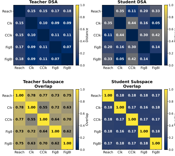
Figure 5: Teacher vs. student dynamics and representational geometry. Pairwise dynamical similarity (DSA distance, top row; lower means more similar dynamics) and principal-subspace overlap (bottom row; mean squared cosine of principal angles between the dominant cortical activity subspaces, higher means more shared geometry) between the five compound tasks, computed for the teacher (left) and the student (right).
