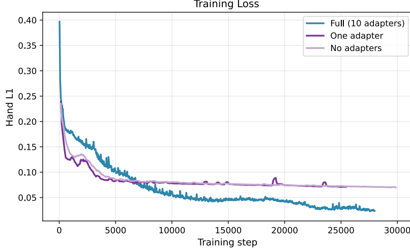
Figure 9: Adapter bank ablation. The previous ablation removed auxiliary supervision components but preserved the adapter architecture. We additionally test whether the adapter bank itself is crucial for the network’s ability to learn the multi-task suite by training two further ablations: one with a single shared adapter ( K=1 , with all tasks routed through the same modulator), and one with no adapters at all (the cortex must learn all task dynamics within a single shared recurrence). For the latter, we allowed the decoder loss to train the LSTM recurrence.
