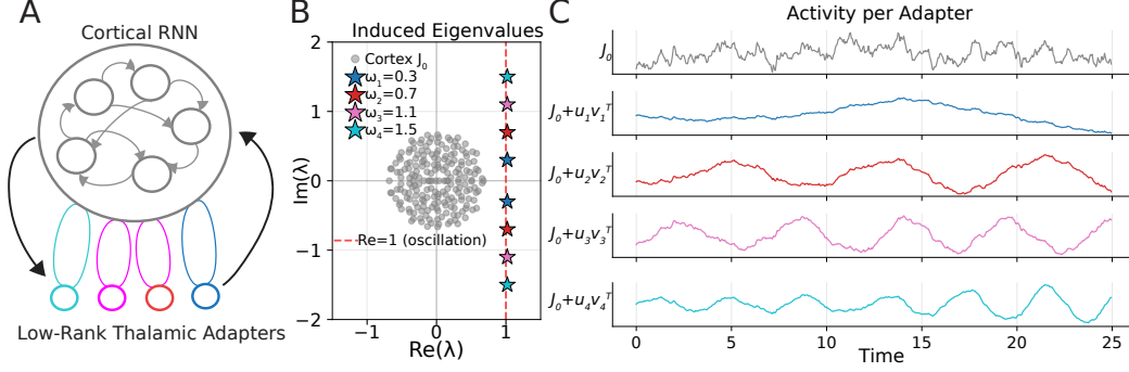
Figure 1: Adapter Banks as Thalamocortical Loops (A) Schematic of the framework of Logiaco et al. [12]: thalamic inputs \mathbf{u}_k drive a cortical RNN with recurrence \mathbf{J}_0 . A rank-one perturbation \mathbf{u}_k \mathbf{v}_k^\top can induce oscillatory dynamics at a target frequency. (B) Eigenvalue placement. Gray: eigenvalues of the bare cortex \mathbf{J}_0 . Stars: target locations on the oscillation line ( \text{Re}(\lambda) = 1 ) for four motifs at different frequencies \omega_k . Each low-rank perturbation shifts a conjugate pair of eigenvalues to the corresponding target. (C) Cortical activity projected onto a one-dimensional readout. Each motif \mathbf{J}_0 + \mathbf{u}_k \mathbf{v}_k^\top sustains a different oscillation at its target frequency \omega_k , demonstrating that rank-one perturbations selectively recruit the cortical network to produce frequency-specific dynamics.
