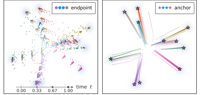
Fig. 4. Visualization of the rectified-flow transport that carries each initial endpoint to its class anchor.
