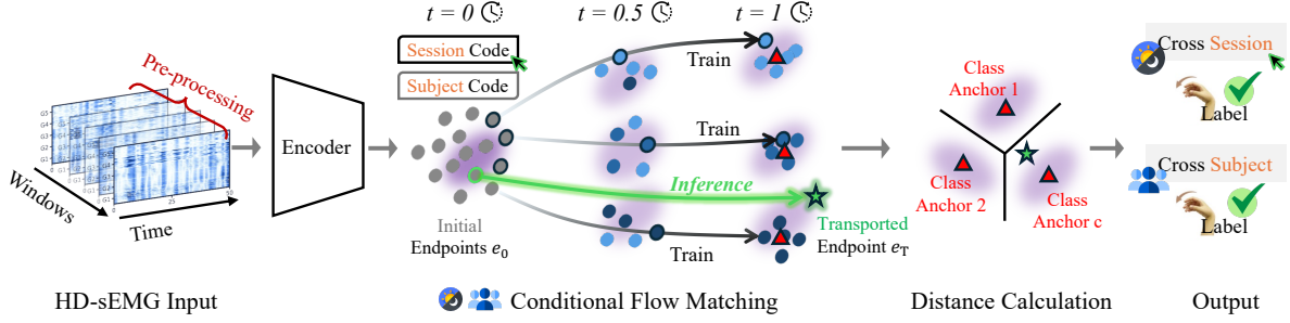
Fig. 1. The framework of the proposed MyoFlow for HD-sEMG gesture recognition across sessions and subjects.
