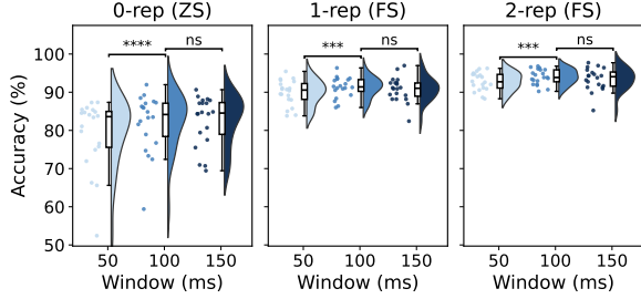
Fig. 2. Temporal-window sensitivity for cross-session recognition on Hyser, with pairwise significance tests.
