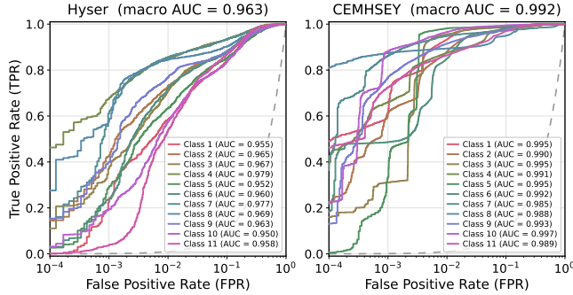
Fig. 3. Zero-shot Receiver Operating Characteristic (ROC) curves of MyoFlow on both datasets. (The FPR is log-scaled)
