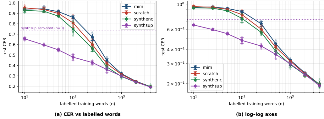
Figure 1: Test CER against the number of real transcribed training words. Panel (a) uses a logarithmic x -axis with a linear y -axis, and panel (b) uses logarithmic axes on both sides. Each point is the mean over six seeds and the bands show the seed standard deviation. At n = 4000 all four arms fall between 0.1924 and 0.1975.
