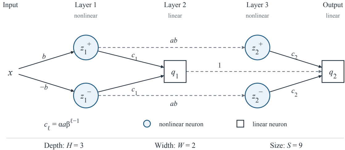
Figure 3.2: An alternating realization of Q_2 , with c_\ell = \alpha a \beta^{\ell-1} . Circles denote nonlinear neurons and squares denote linear neurons. Dashed skip connections carry the branch values and the running sum across one intervening layer. All three hidden layers contribute to depth.
