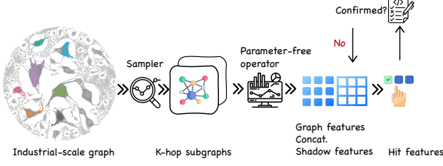
Figure 4: GraphFAS procedure overview.
