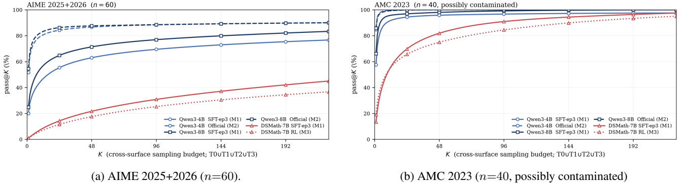
Figure 9: Cross-mechanism pass@K pooled across T0+T1+T2+T3 ( K_{\max}=224 )
