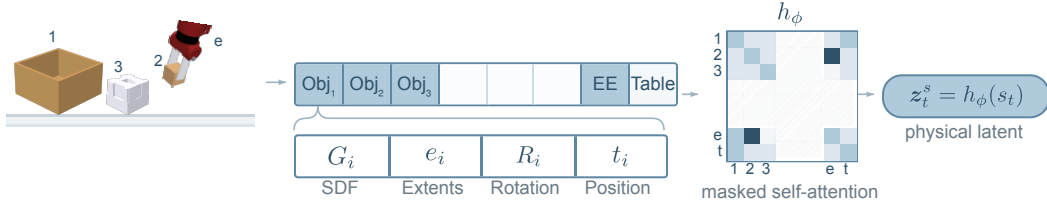
Figure 3: Each scene is represented by object, end-effector, and table tokens under a shared schema. The physical encoder ( h_\phi ) first applies masked self-attention over the valid scene tokens, then uses a learned query to attend to and pool the token set into a single physical latent ( z_t^s ). Unused object slots are masked in both stages, allowing the same encoder to process scenes with different numbers of objects.
