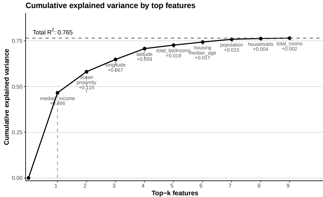
Figure 5: Cumulative feature-specific R^2 values of the top-ranked features for the California housing data.
