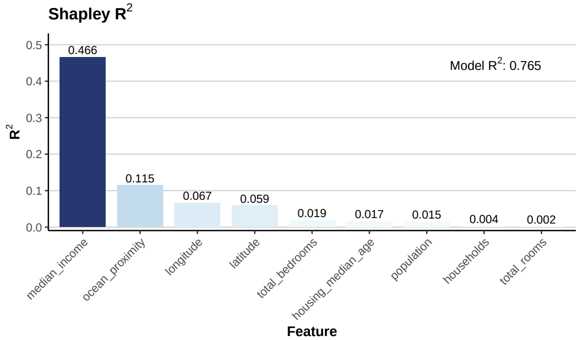
Figure 2: Feature-specific R^2 values for the California housing data.
