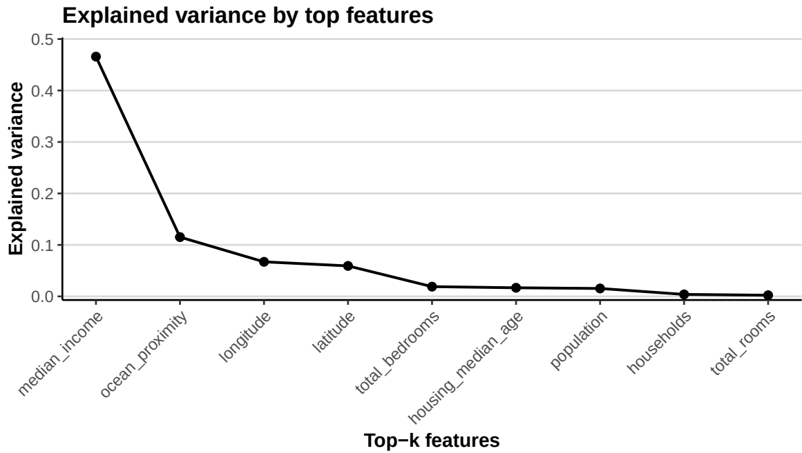
Figure 4: Elbow plot of feature-specific R^2 values for the California housing data.
