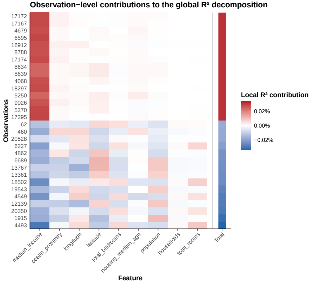
Figure 6: Observation-level contributions to the global R^2 decomposition for selected observations.
