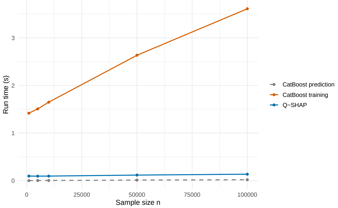
Figure 1: Runtime scaling of CatBoost fitting, prediction, and qshap as the number of explained samples increases, averaged over 10 replications. The feature dimension is fixed at p = 100 , and CatBoost is trained with K = 100 trees. Prediction time is included for reference.
