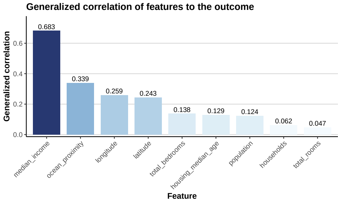
Figure 3: Feature-specific generalized correlation coefficients for the California housing data.
