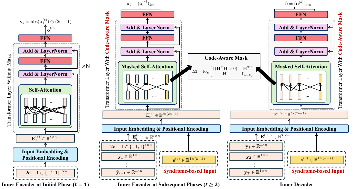
Fig. 4. Overall schematic diagram of encoder/decoder of MASKCODE. (Left) The inner encoder at initial phase ( t = 1 ) processes the bipolar-mapped codeword using a standard Transformer. (Middle) The inner encoder at subsequent phases ( t \geq 2 ) utilizes the code-aware mask derived from the parity check matrix \mathbf{H} and the soft syndrome-based input to refine parity messages based on noisy feedback. (Right) Similar to the inner encoder, the inner decoder aims to produce reliable LLRs to the outer decoder by aggregating received parity messages, as well as the soft syndrome-based input corresponding to the initial-phase parity message.
