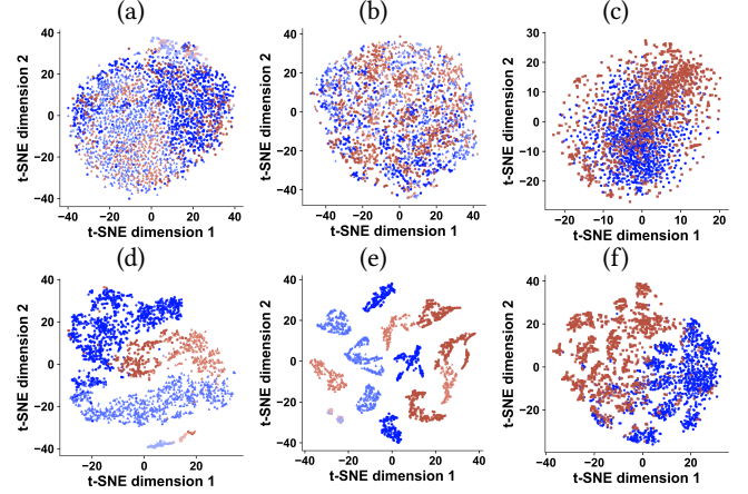
Figure 5: t-SNE of standardized SAGE perturbation representations. Panels (a–c) use classification and panels (d–f) use TASSO on PROTEINS_full, ENZYMES, and Cora, respectively. Panels (c) and (f) show Hadamard link-pair features; colors and marker shapes denote LP labels.
