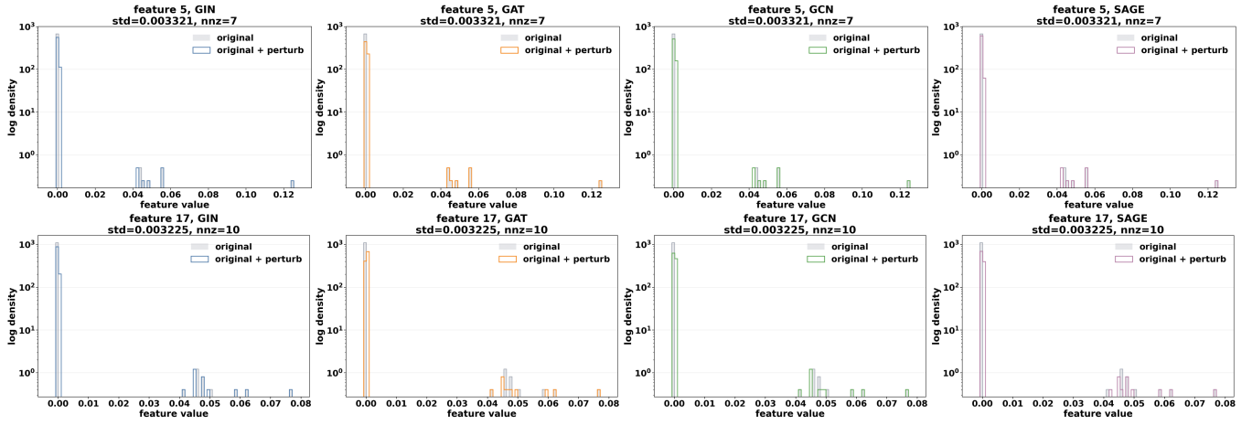
Figure 10: Original versus perturbed feature-value histograms for Cora, shown for representative features. The logarithmic y-axis improves visibility of low-frequency nonzero values because the original feature values are highly concentrated near zero.
