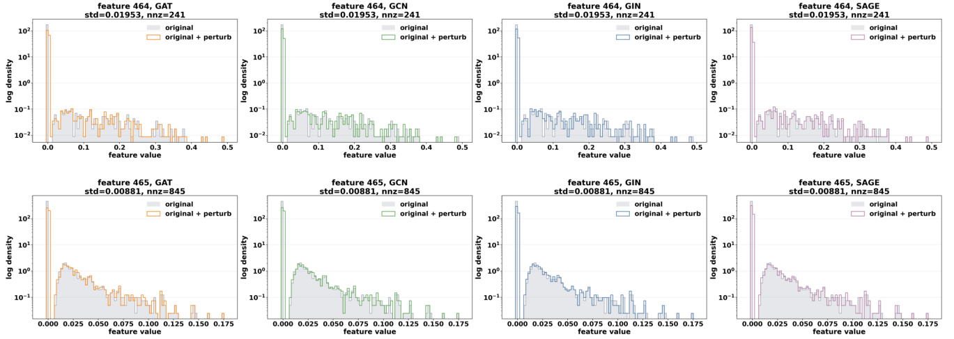
Figure 11: Original versus perturbed feature-value histograms for PubMed, shown for representative features.
