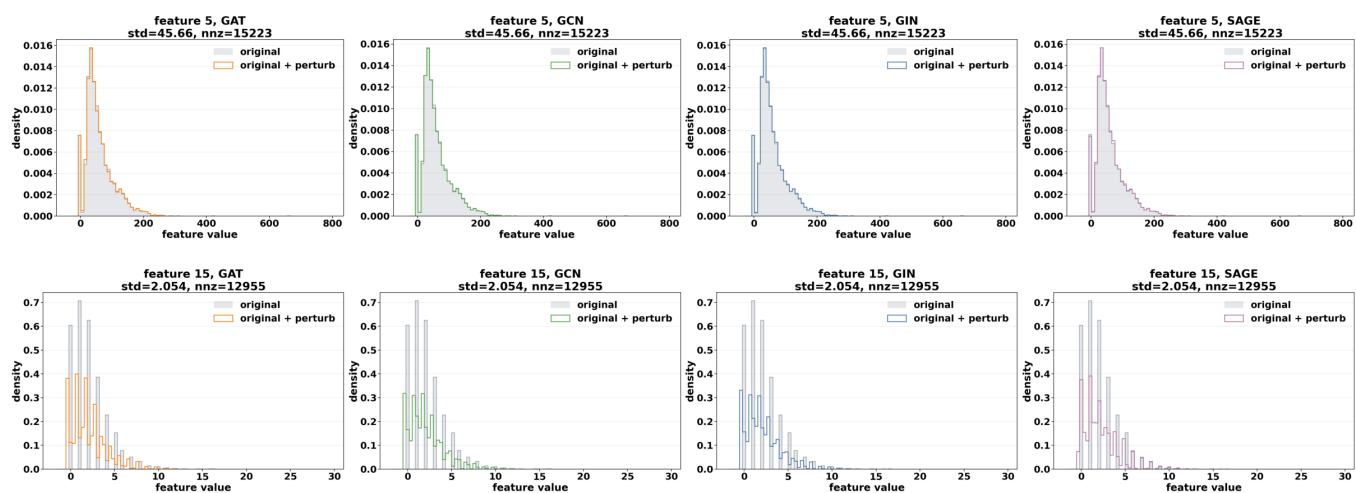
Figure 12: Original versus perturbed feature-value histograms for ENZYMES, shown for representative features.
