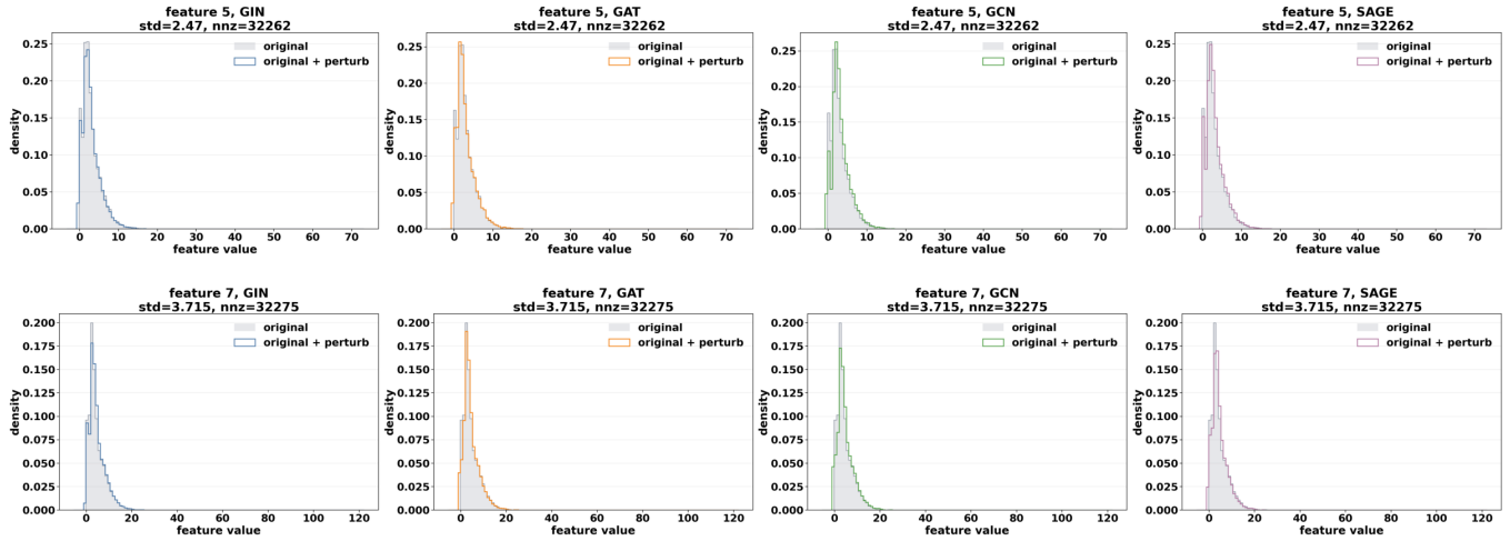
Figure 9: Original versus perturbed feature-value histograms for PROTEINS_full, shown for representative features.
