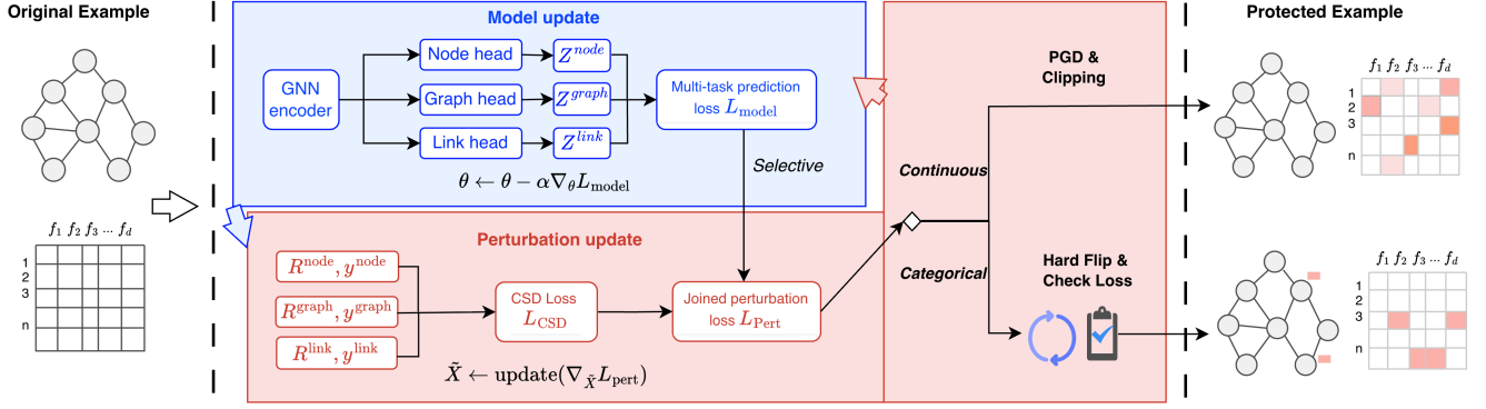
Figure 2: Overview of MUGEN. We alternate GNN updates using the enabled-task prediction losses and perturbation updates. Continuous attributes use clipped PGD, whereas categorical attributes use hard flips with exact loss evaluation.
