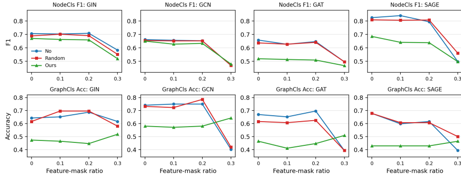
Figure 6: Complete feature-masking robustness results on PROTEINS_full. Panels show node F1 and graph accuracy for clean data (No), Gaussian random perturbations (Random), and perturbations generated by our framework (Ours).
