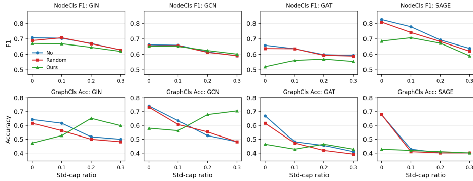
Figure 8: Complete adversarial-training robustness results on PROTEINS_full. Panels show node F1 and graph accuracy for clean data (No), Gaussian random perturbations (Random), and perturbations generated by our framework (Ours).
