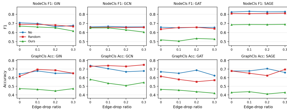
Figure 7: Complete edge-dropping robustness results on PROTEINS_full. Panels show node F1 and graph accuracy for clean data (No), Gaussian random perturbations (Random), and perturbations generated by our framework (Ours).
