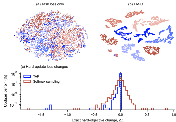
Figure 1: Perturbation representations produced by (a) the task loss and (b) TASO. Color denotes graph class and shape denotes node class. (c) Softmax sampling frequently increases the perturbation loss ( \Delta L > 0 ), whereas TAP’s hard-coordinate updates ensure non-increasing loss ( \Delta L \leq 0 ).
