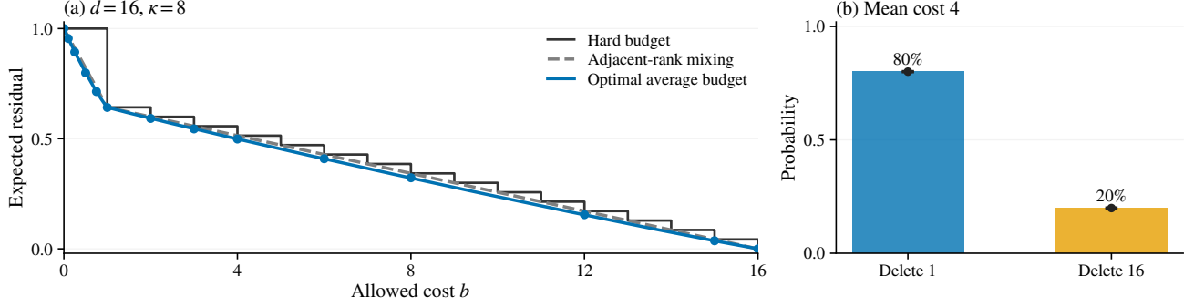
Figure 5: An average budget rewards adaptive deletion rank. Left: exact hard-budget, adjacent-rank mixing, and optimal average-budget risks at d = 16, \kappa = 8 , with points from 131,072 shared draws. Right: at average cost four the optimal rule deletes one direction with probability 0.8 and all sixteen with probability 0.2. Black points with exact 95% binomial intervals check these probabilities.
