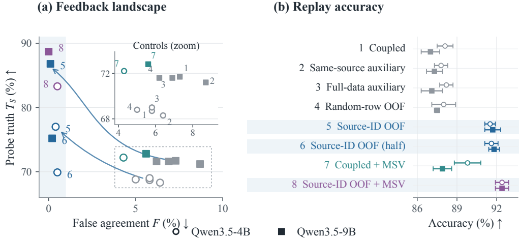
Figure 7: Mechanism ablations on a fixed replay bank. (a) Truth versus false agreement; arrows compare coupled and source-ID feedback. (b) Accuracy on 3,000 replay questions, mean \pm SD over five seeds. Numbers identify methods; shading marks source exclusion.
