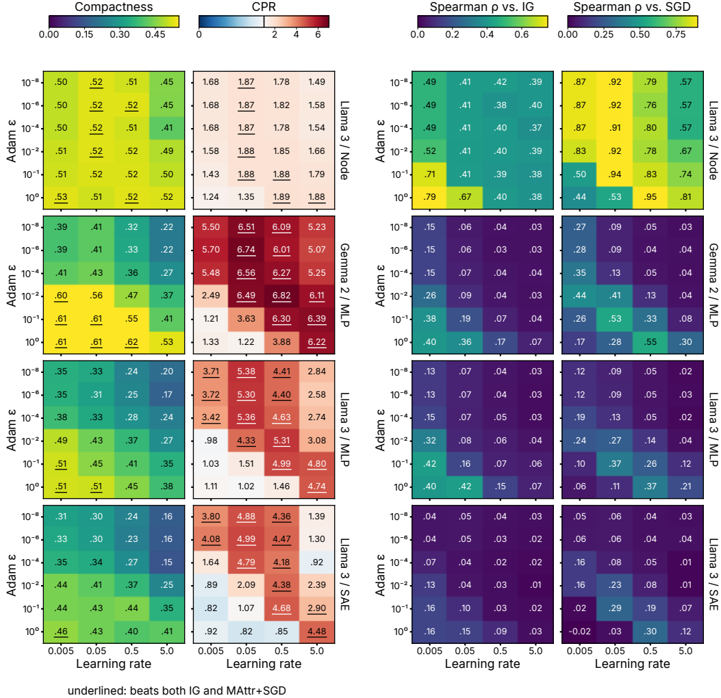
(a) Compactness and CPR; underlined cells beat both IG and MATtr+SGD on that basis. (b) Spearman \rho of the learned ranking against IG and against MATtr+SGD at its own best learning rate.
