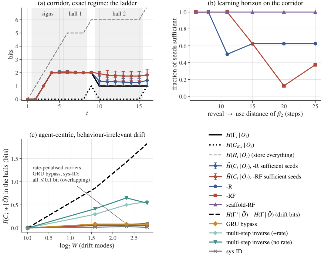
Figure 6: Signpost corridor. (a) In the exact regime at M = 16 , sufficient seeds carry 2.00 bits through hall 1 while H(G_{E,t} | \bar{O}_t) = 0 , then reduce their rate after junction 1; the history contains 5 bits. Expiration is partial (1.2–1.8 compared with 1.0). (b) Fraction of sufficient seeds as a function of the reveal → use distance for \beta_2 (hall-2 length 1–20). The plain realizations decay with distance (logit slope -0.11/\text{step} , p = 0.01 with configuration-clustered errors), whereas the annealed scaffold does not. (c) Drift information retained in the halls as a function of \log_2 W . The multi-step-inverse memory carries 0.3–0.7 bit about the drift, with or without the rate term, whereas DIACRITIC and system identification carry \leq 0.08 bit. The dashed line denotes the additional rate assigned by the strong congruence.
