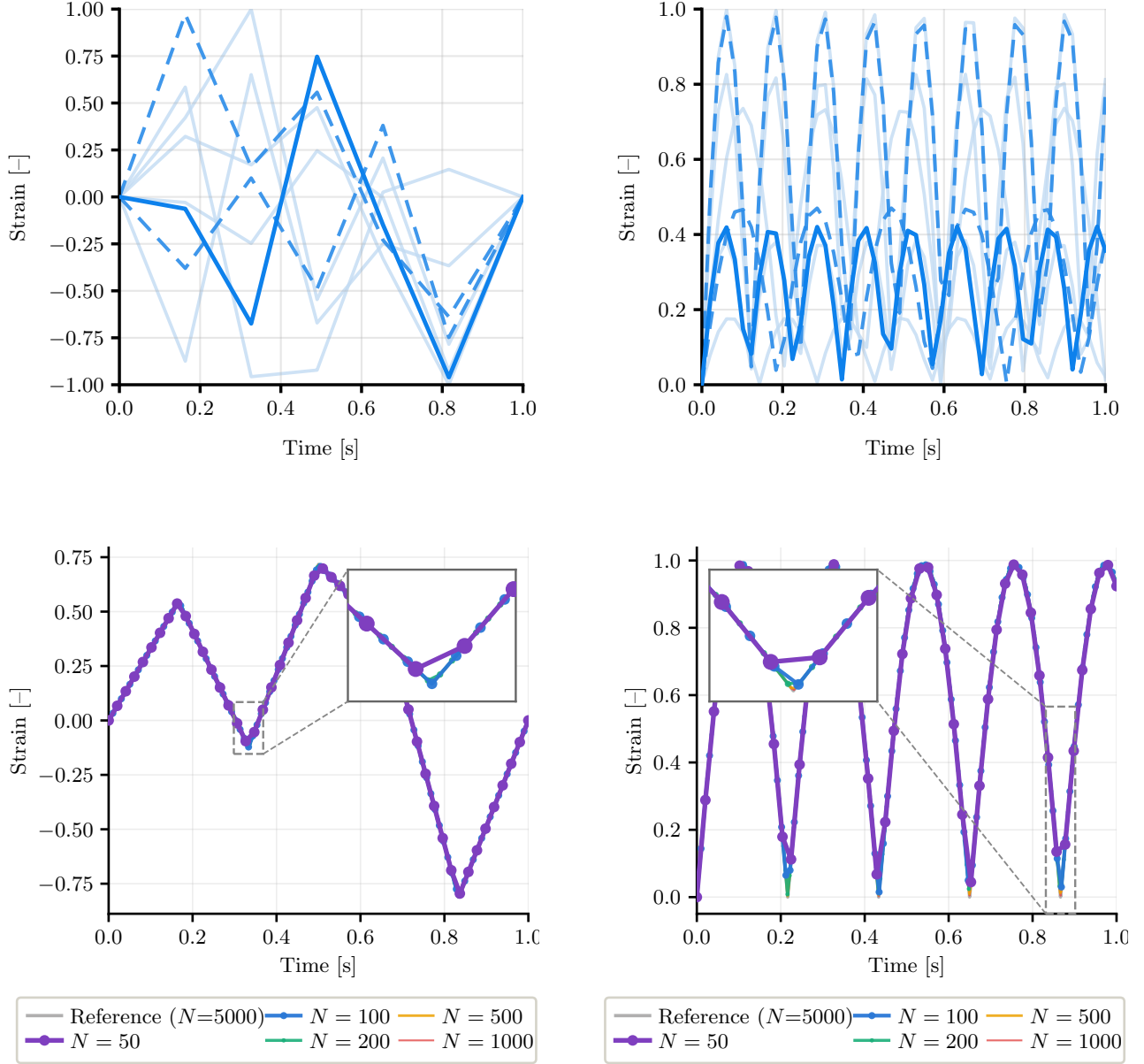
Figure 7: Testing distribution and discretization study. Top row shows sample strain paths from the two testing distributions, zig-zag (left) and sinusoidal (right), with bold and dashed curves marking representative examples among the faint background paths. Bottom row shows the same paths resampled at different resolutions ( N = 50 to N = 1000 ) against a high resolution reference ( N = 5000 ).
