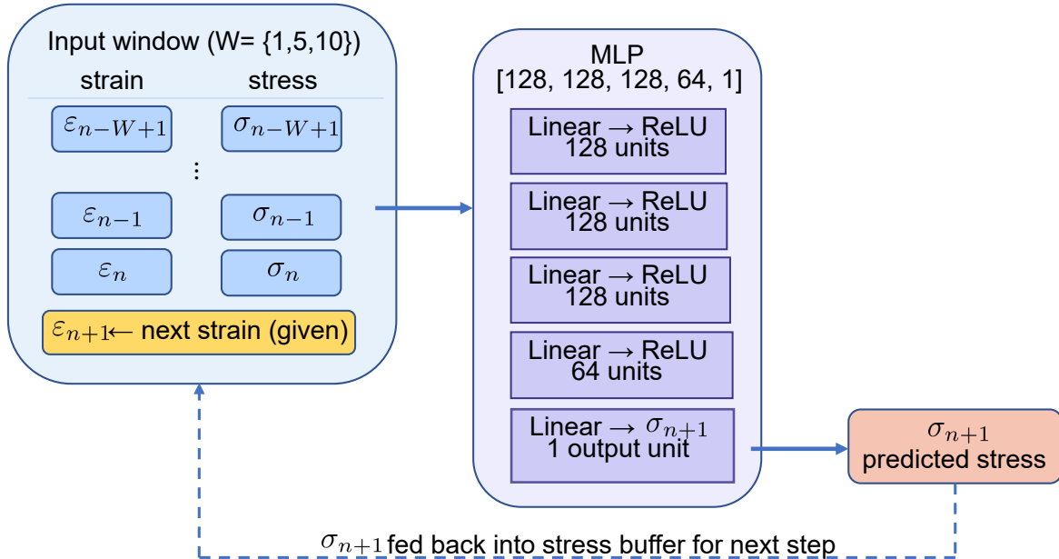
Figure 4: Autoregressive Inference: Feed Forward Neural Network Architecture
