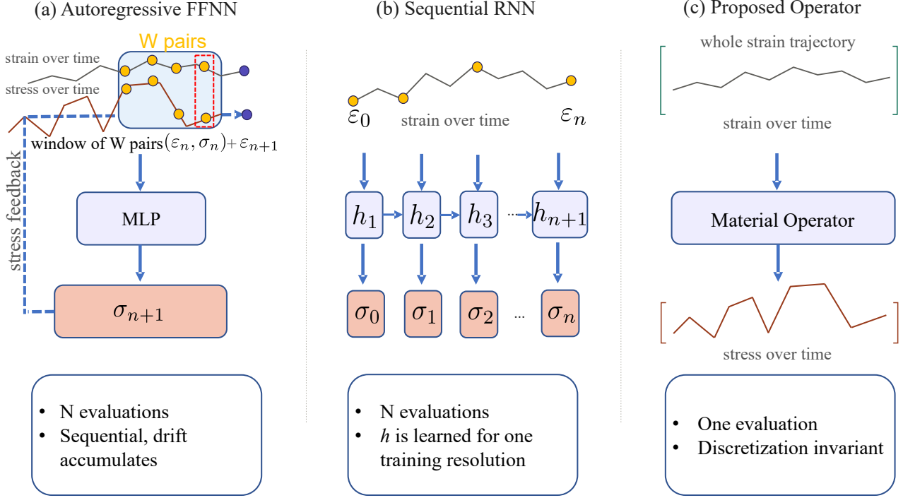
Figure 1: Three paradigms for data-driven path-dependent constitutive modeling at inference time (a) Autoregressive FFNN (b) Sequential RNN-GRU (c) Proposed material operator
