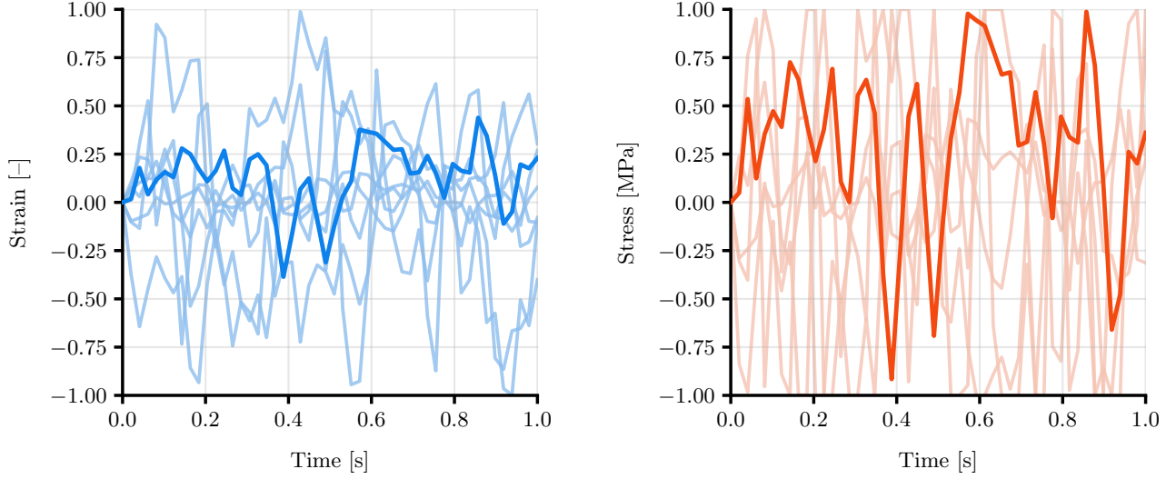
Figure 6: Training distribution of strain paths (blue, left) and corresponding stress responses (orange, right). The bold solid curves highlight representative strain–stress pairs, while the faint curves are some remaining trajectories in the dataset.
