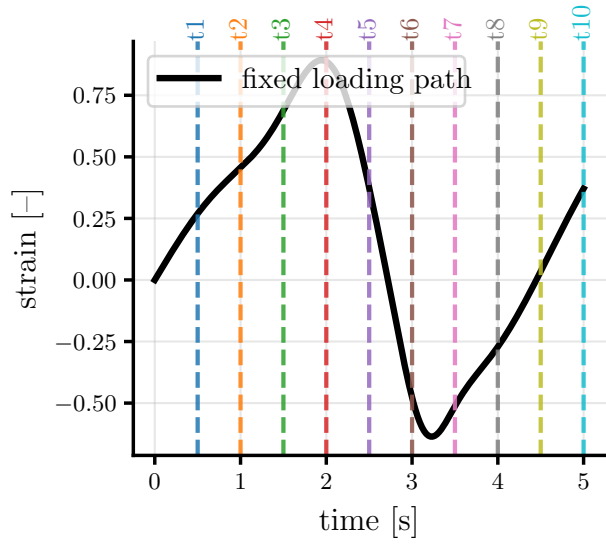
(a) Input strain
