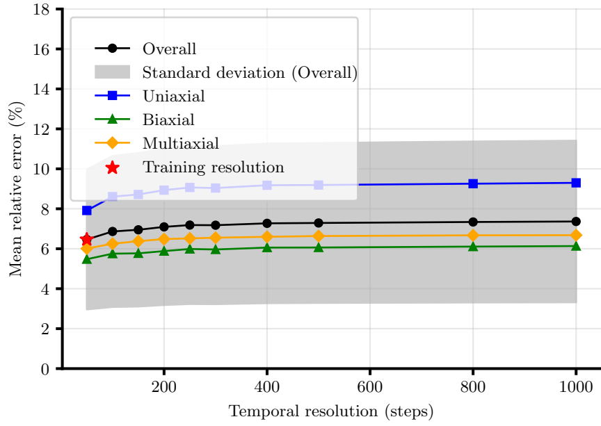
(b) FNO-SIREN
