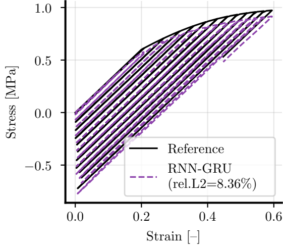
(c) RNN-GRU
