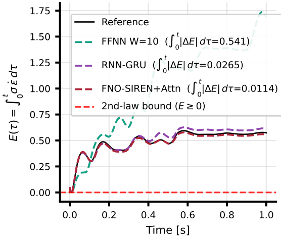
(e) Mechanical work for 1D coupled damage-plasticity model
