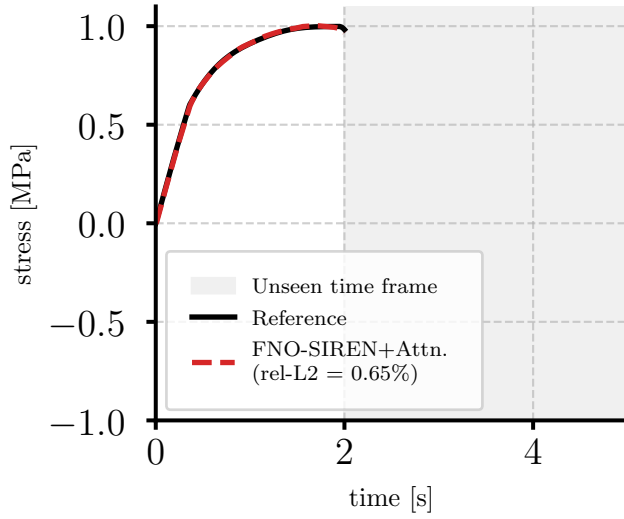
(c) Stress field till t4 (2 s)
