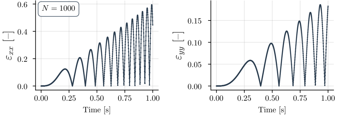
(a) Strain loading path at temporal resolution N = 1000
