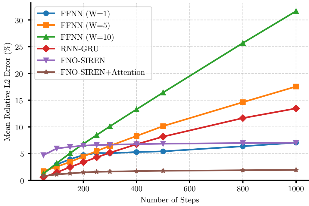
Figure 21: Discretization study on sinusoidal loading paths, 1D elastoplastic material model.
