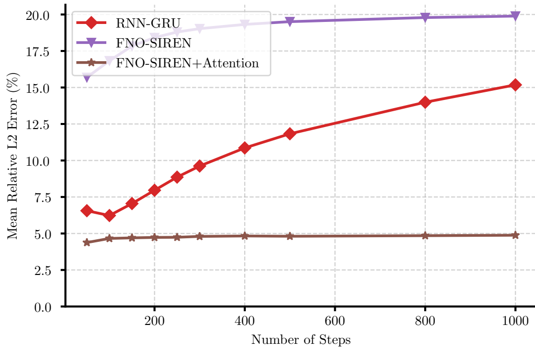
Figure 23: Discretization study on sinusoidal loading paths, 1D coupled damage-plasticity model.
