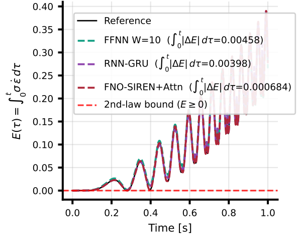
(d) Mechanical work for 1D elastoplasticity material model
