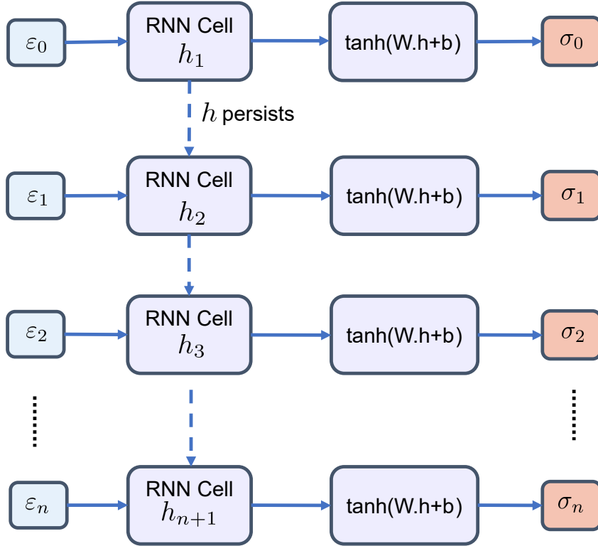
Figure 5: RNN architecture variant with GRU cell
