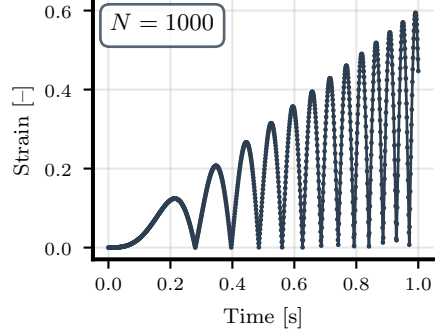
(b) Complex loading path at higher resolution
