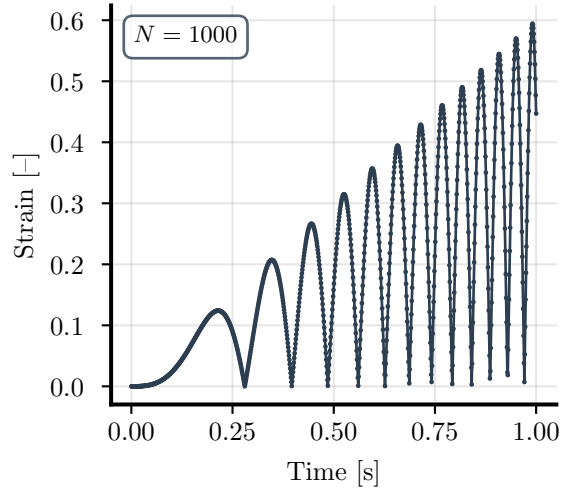
(a) Strain loading path at temporal resolution N = 1000
