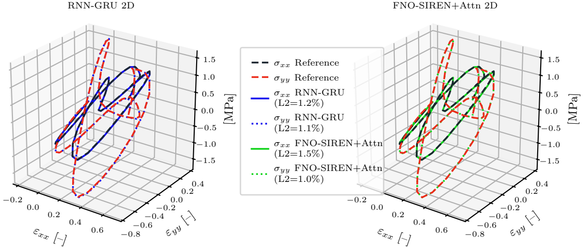
Figure 16: In-distribution(Gaussian-Process) loading path at temporal resolution N = 50
