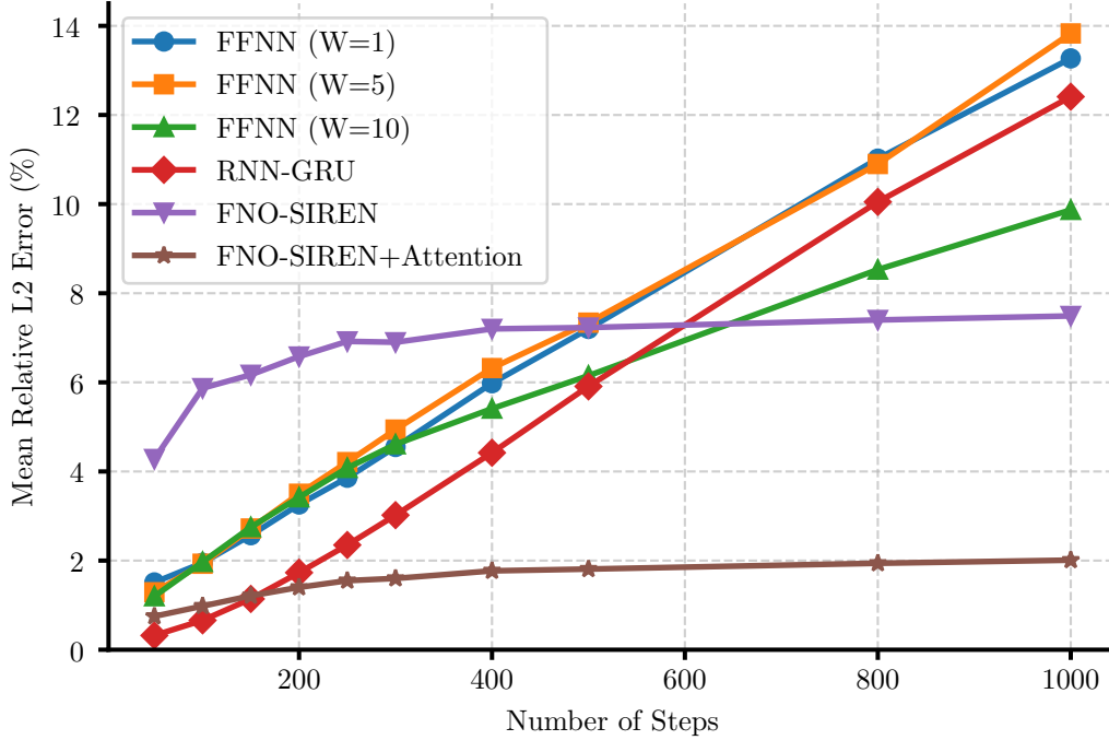
Figure 11: Discretization Study - Comparison Plot
