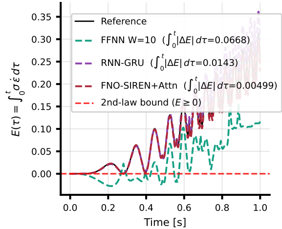
(f) Mechanical work for 1D coupled damage-plasticity model
