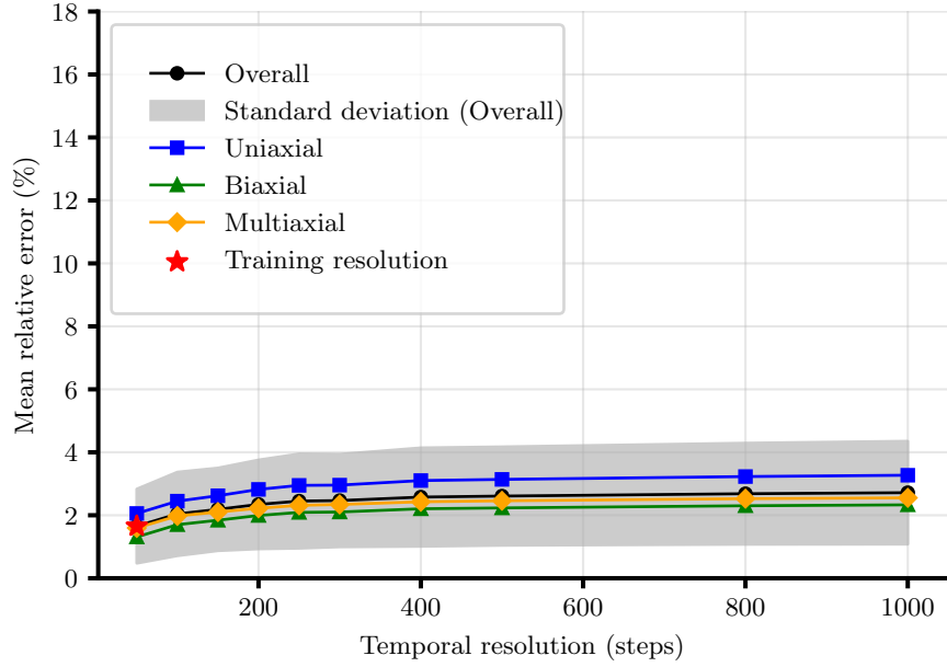
(c) FNO-SIREN+Attention
