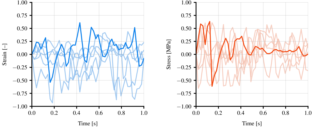
Figure 12: Training distribution: strain paths with corresponding stress paths
