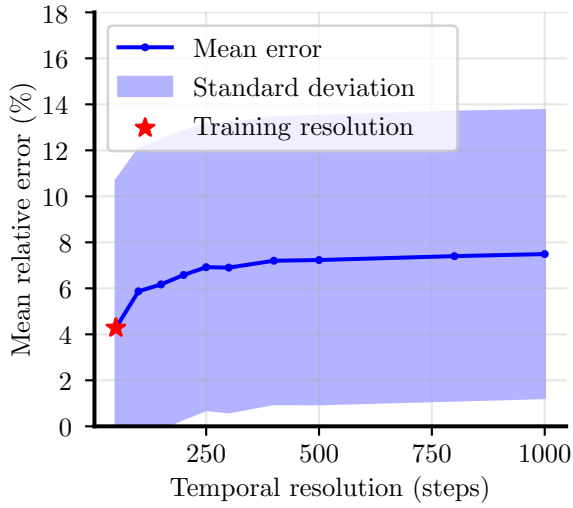
(e) FNO-SIREN
