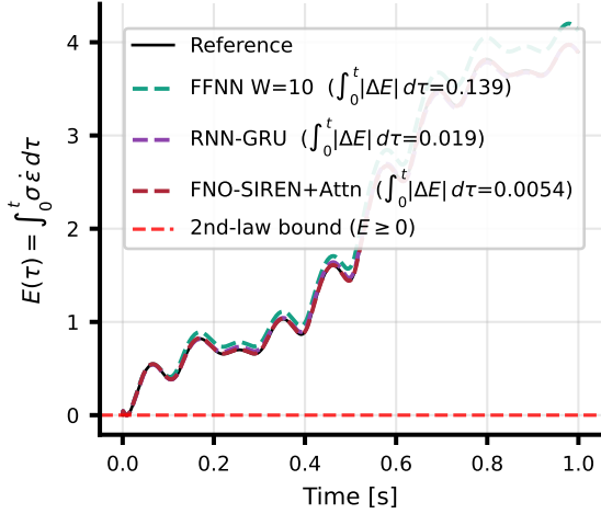
(c) Mechanical work for 1D elastoplasticity material model
