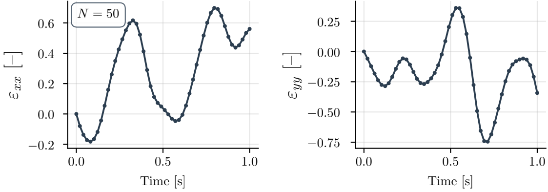
(a) Strain loading path at training resolution
