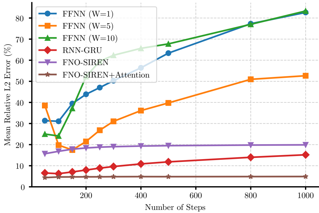
Figure 22: Discretization study on sinusoidal loading paths, 1D coupled damage-plasticity model.
