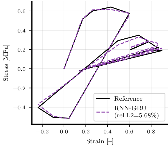
(c) RNN-GRU
