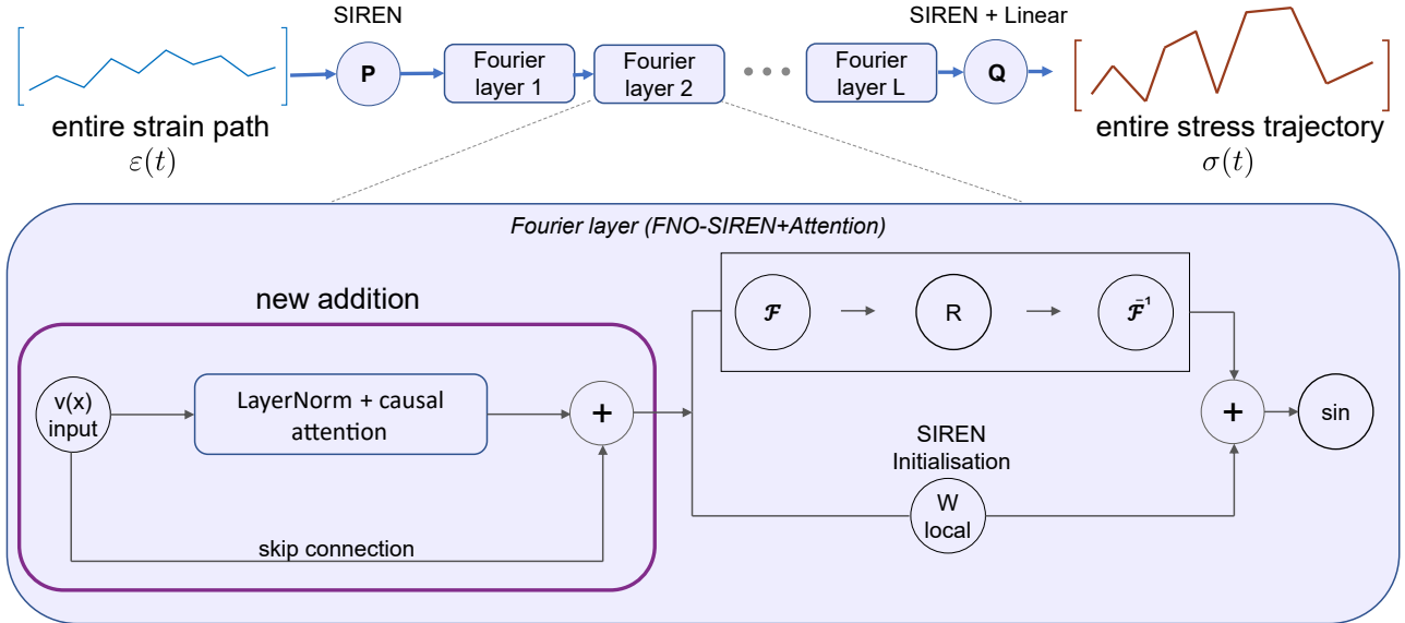
Figure 2: FNO-SIREN+Attention
