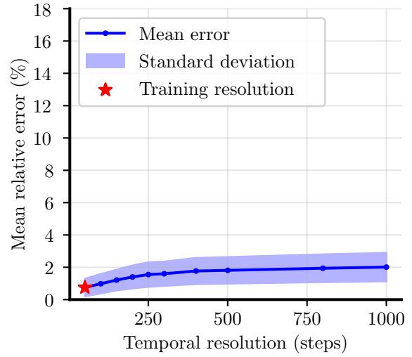
(f) FNO-SIREN+Attention
