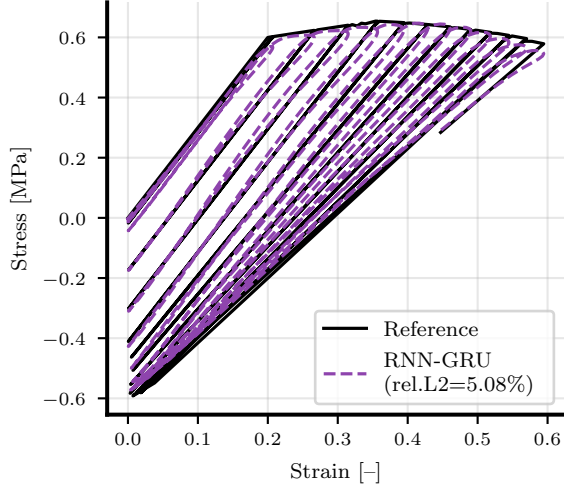
(c) RNN-GRU
