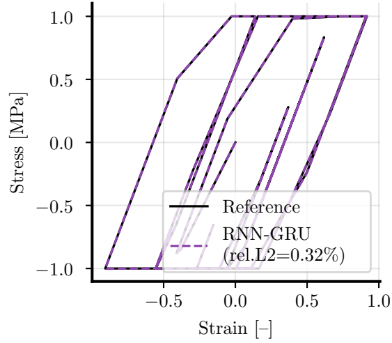
(c) RNN-GRU
