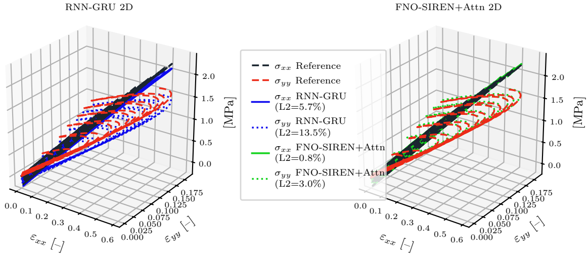
Figure 17: Complex loading path at temporal resolution N = 1000
