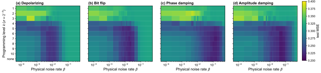
Figure 4. Testing error across physical noise rates and noise-programming levels. Mean testing MSE after training at physical noise rate \beta and programming level k , corresponding to a parameter-perturbation strength \sigma = 2^{-k} . The row labelled “none” is the unprogrammed baseline. Each cell is averaged over ten runs.
