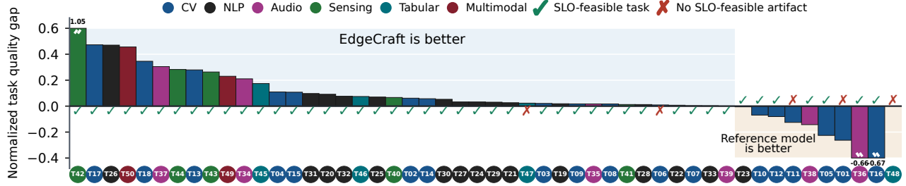
Figure 8: Normalized task quality gap of EdgeCraft and reference models on 50 edge/mobile datasets.
