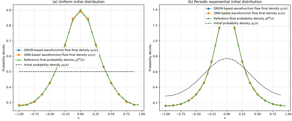
Fig. 15 Comparison of final probability densities generated by wavefunction flow simulation using QNN and QROM-based phase kickback frameworks, and reference final densities under V_2(x, t)
