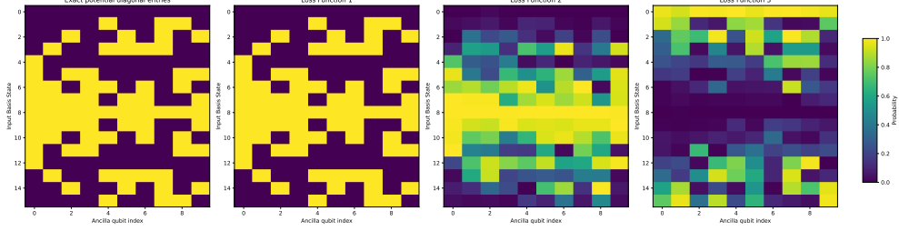
Fig. 13 The comparison between the binary representations of the exact potential diagonal entries of D_{V_{t_0}} and the corresponding probabilities learned by the QNN circuit under different loss functions. The y -axis represents the states of the input, where each state corresponds to a diagonal entry. The x -axis represents the ancilla qubit indices, where the i -th qubit index corresponds to the i -th binary bit of the diagonal entry
