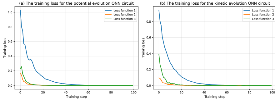
Fig. 12 The training losses for the potential and kinetic evolution QNN circuits with different loss functions
