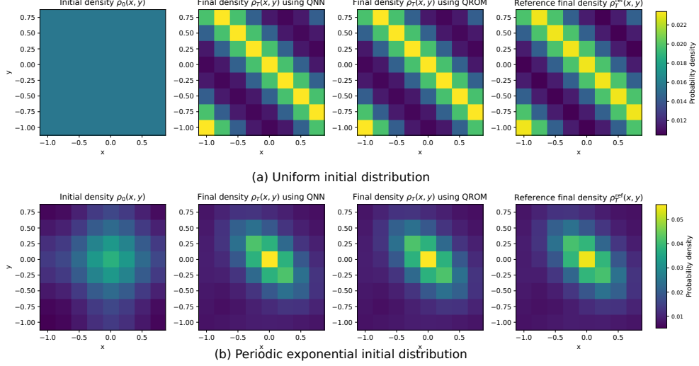
Fig. 17 Comparison of final probability densities generated by wavefunction flow simulation using QNN- and QROM-based phase kickback frameworks, and reference final densities under V_4(x, y, t)
