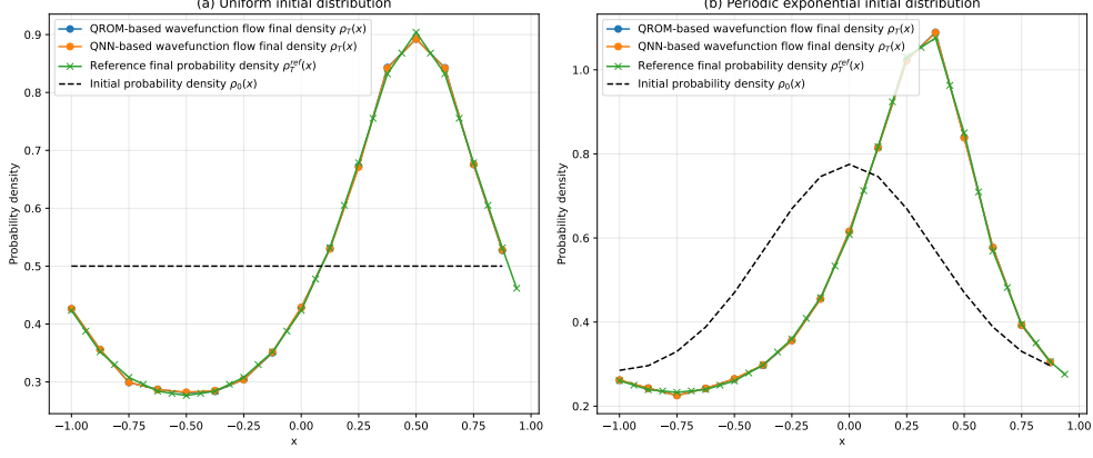
Fig. 14 Comparison of final probability densities generated by wavefunction flow simulation using QNN- and QROM-based phase kickback frameworks, and reference final densities under V_1(x, t)
