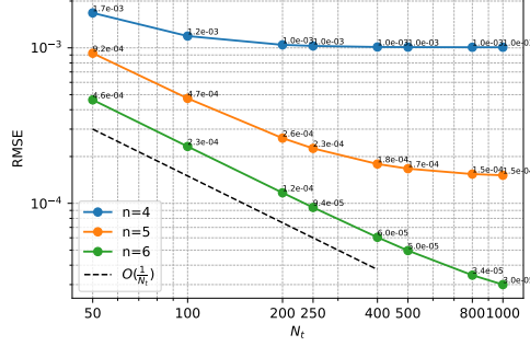
Fig. 21 Errors between the final probability densities generated by the wavefunction flow simulation and reference final probability densities with different N_t under different numbers of address qubits
