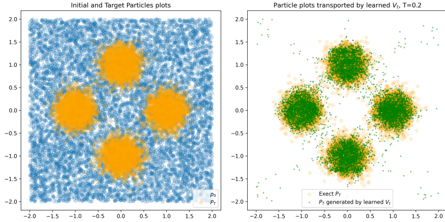
Fig. 22 The left figure shows the initial and the target particle plots. The right figure shows the final particle plot obtained by the flow model, in which the particles are transported under the velocity field generated by the learned potential V_t through flow matching, together with the exact target particle plot
