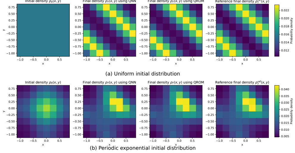
Fig. 16 Comparison of final probability densities generated by wavefunction flow simulation using QNN- and QROM-based phase kickback frameworks, and reference final densities under V_3(x, y, t)
