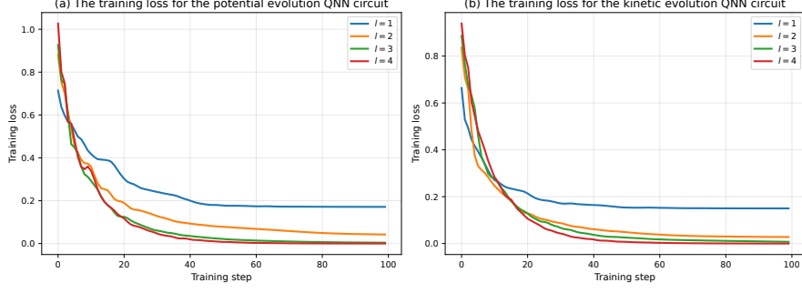
Fig. 11 The training losses for the potential and kinetic evolution QNN circuits with different numbers of layers l
