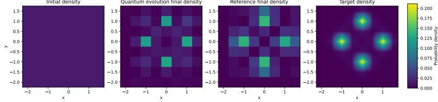
Fig. 23 Comparison of the final probability density obtained by wavefunction flow simulation and the target distribution. The first figure represents the initial probability density, the second figure denotes the final probability density obtained by the wavefunction flow simulation, the third figure shows the the corresponding reference final density, and the last figure shows the target probability density consisting of four Gaussian balls
