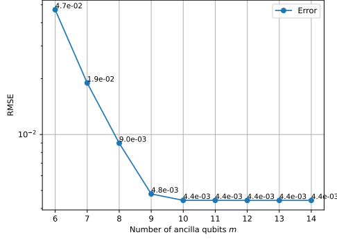
Fig. 19 Errors between the final probability densities generated by wavefunction flow simulation and the reference final probability densities with different numbers of ancilla qubits m
