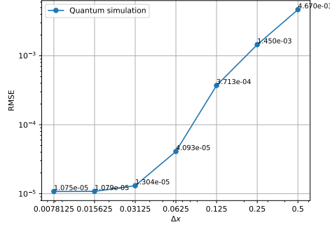
Fig. 20 Errors between the final probability densities generated by wavefunction flow simulation and reference final probability densities with different \Delta x
