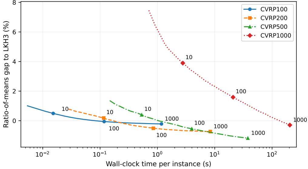
Figure 3: Anytime quality–runtime trade-off of S3 with polar RRC. The x-axis shows wall-clock time per instance on a logarithmic scale; markers are labeled by reconstruction iteration (10, 100, and 1,000). The y-axis is the ratio-of-means gap to the LKH3 references computed from the saved incumbent-cost trajectory. Lower is better.
