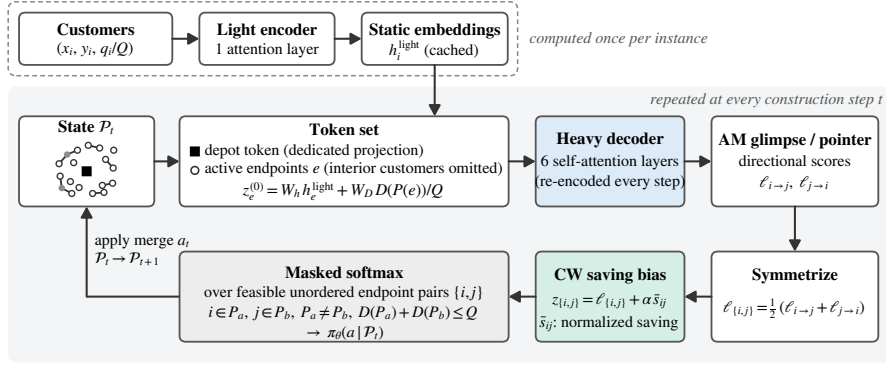
Figure 2: Policy architecture. Static customer features are encoded once by a light encoder. At each construction step, the depot token and active endpoints, together with their component loads, are re-encoded by the heavy decoder. An AM-based glimpse/pointer produces directional scores, which are symmetrized into unordered pair scores, augmented by the normalized CW-saving bias, and normalized by a masked softmax over capacity-feasible endpoint pairs. Applying the selected merge produces the next component state. For clarity, the graph-context term used in the full implementation is omitted; the endpoint-token equation is the conceptual form of Section 3.4.
