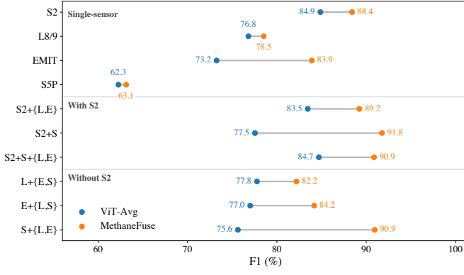
Fig. 5. Sensor-set transfer at the 480 m footprint measured by F1. Rows are grouped into single-sensor, S2-present, and S2-absent regimes. L, E, and S denote L8/9, EMIT, and S5P.
