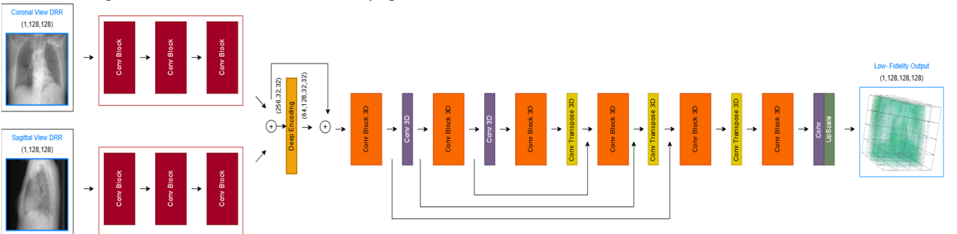
Figure 4 Network architecture used for the DRR-to-CT transformation in the first pass. The 2D convolutional block (Conv Block 2D) consists of two sequential Conv2D–Batch Normalization–ReLU layers, while the 3D convolutional block (Conv Block 3D) consists of two sequential Conv3D–Batch Normalization–ReLU layers.
