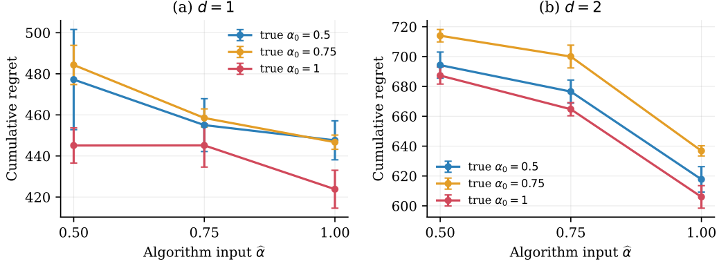
Figure 4: Sensitivity to smoothness mismatch at T = 8000 . Each curve fixes the true cusp exponent \alpha_0 and varies the algorithm input \hat{\alpha} ; points are means over six common-random-number repetitions and error bars are 95% confidence intervals. Left: d = 1 . Right: d = 2 .
