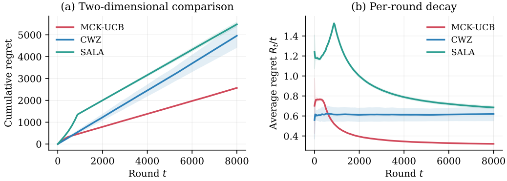
Figure 3: Two-dimensional comparison with neighboring online joint pricing–inventory methods under common exogenous context and residual-shock trajectories. Curves are means over eight repetitions and shaded regions are 95% confidence intervals. CWZ and SALA are noncontextual prior-work baselines and pool away the context, whereas MCK-UCB uses contextual kernel estimates.
