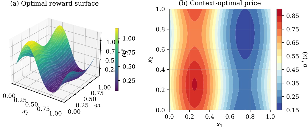
Figure 2: Geometry of the two-dimensional instance used in the baseline comparison. Left: optimized reward G_x^* = \max_p G_x(p) . Right: context-optimal price p^*(x) . The substantial price variation makes context information decision relevant.
