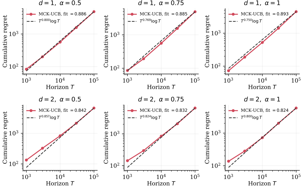
Figure 1: Cumulative-regret scaling of the paper-aligned MCK-UCB policy for different context dimensions d and Hölder exponents \alpha . Solid curves are means over five exogenous trajectories, shaded regions are 95% confidence intervals, and dashed curves give representative T^{\beta(d,\alpha)} \log T guides.
