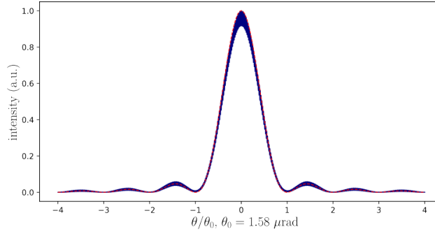
Figure 19: Far-field intensity distribution ( L = 10 km, N_F = 0.11 ): the solid line shows the numerical result in normalized angular coordinate \theta/\theta_0 . The dashed line shows the theoretical \text{sinc}^2(\pi W_\perp \theta/\lambda) .
