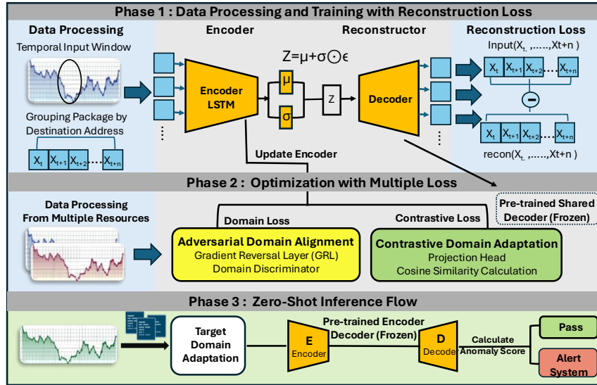
Figure 1: Overall architecture of the proposed Contrastive Adversarially-Adaptive LSTM-VAE framework. The model is trained using two unlabeled source datasets to learn domain-invariant and semantically structured latent representations. Adversarial learning minimizes the domain discrepancy through a gradient reversal layer and domain classifier, while contrastive loss refines the latent space geometry. Adaptors normalize cross-domain input/output formats. At inference, the model generalizes to the unseen target domain in a zero-shot manner using reconstruction error and latent deviations for anomaly detection.
