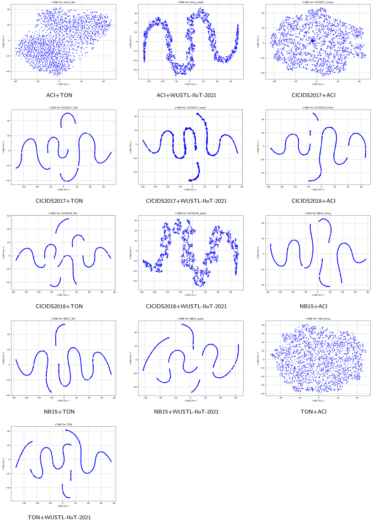
Figure 5: Phase 2 latent space visualization after contrastive and adversarial alignment. Each panel shows the t-SNE projection of the aligned VAE latent representations for one source domain pair.
