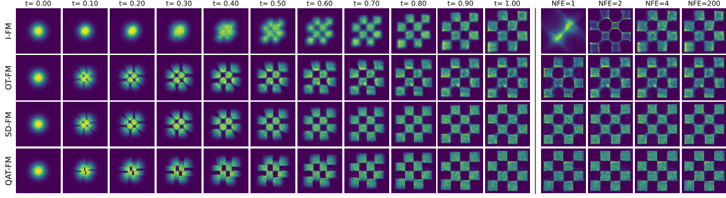
Figure 2: 2D checkerboard results. (Left) sample evolution induced by different coupling methods from t = 0 to t = 1 . (Right) generated samples with varying numbers of function evaluations (NFE).
