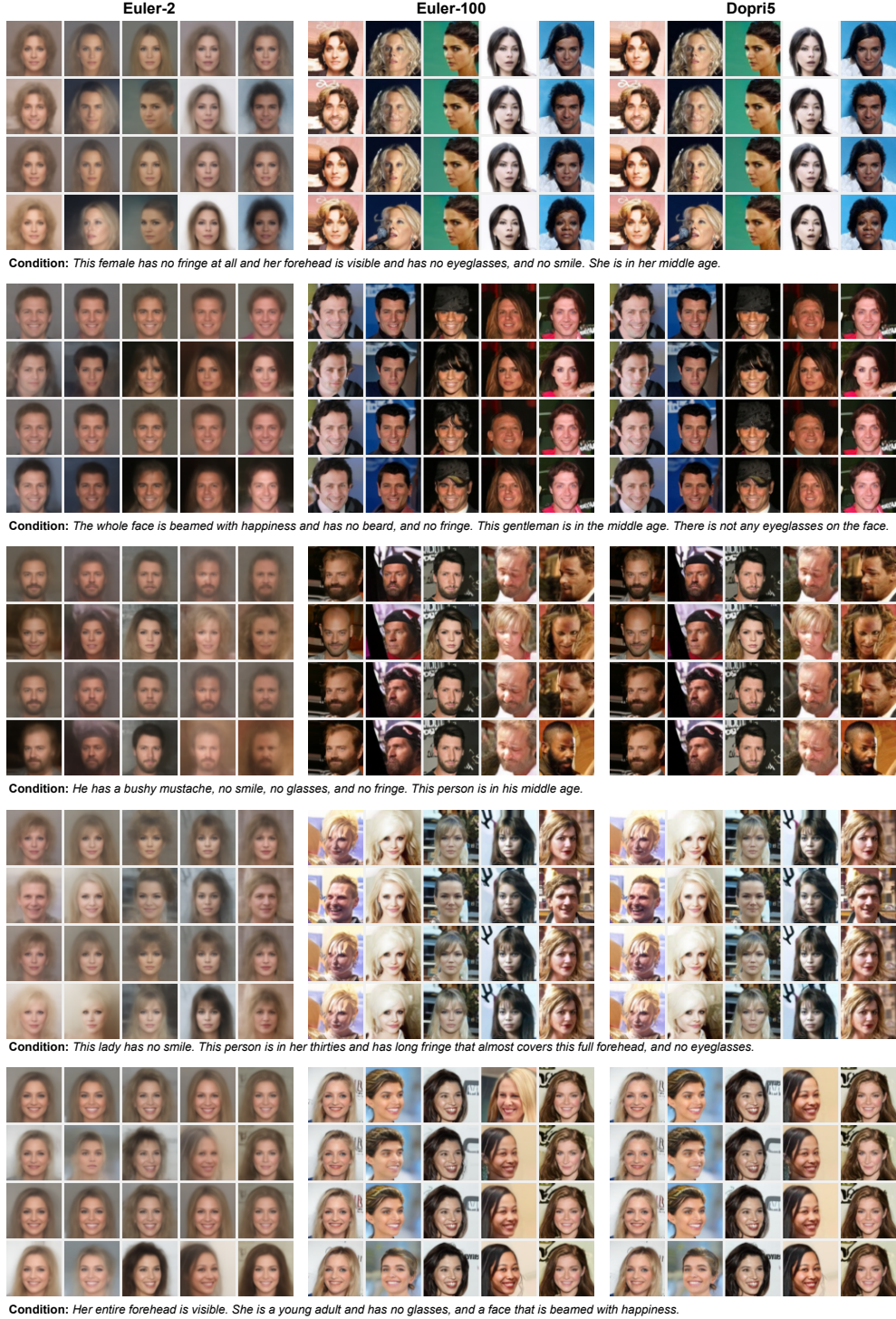
Figure 9: Additional generated samples for text-conditional CelebA-64 \times 64 generation. Each horizontal block corresponds to one CelebA-Dialog text condition; the three columns show results under Euler-2, Euler-100, and Dopri5; within each block, the four rows correspond to I-FM, OT-FM, C2OT and QAT-FM. All images are randomly generated without cherry-picking.
