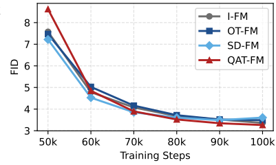
Figure 3: FID (Dopri5) vs. steps.
