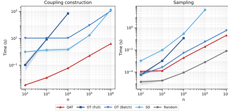
Figure 6: Runtime comparison of different coupling strategies. Left: total coupling construction time over 100 epochs. Right: total sampling time over 100 epochs.
