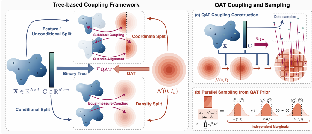
Figure 1: Overview of the QAT coupling and sampling procedure. (Left) QAT builds a binary partition tree over the data using feature-based or condition-aware splits, and transfers the same tree topology to the Gaussian source by quantile alignment, yielding the structured coupling \pi_{\text{QAT}} . (Right) each data leaf is paired with an aligned Gaussian source region. Since these source regions are axis-aligned hyperrectangles, sampling from the corresponding QAT conditional reduces to parallel per-coordinate truncated normal sampling.
