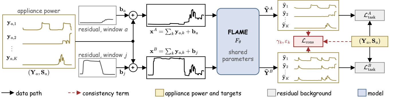
Fig. 2. Label-preserving aggregate recomposition and training objective. The appliance power of window a is added to its own residual background \mathbf{b}_a and to that of another recorded window j , giving two aggregates that differ only in the residual background (11) and share the targets (\mathbf{Y}_a, \mathbf{S}_a) ; one model predicts both windows under the full task loss, and \mathcal{L}_{\text{cons}} uses predictions of the same pair from a second forward pass with dropout disabled. Traces: Reference Energy Disaggregation Data Set (REDD).
