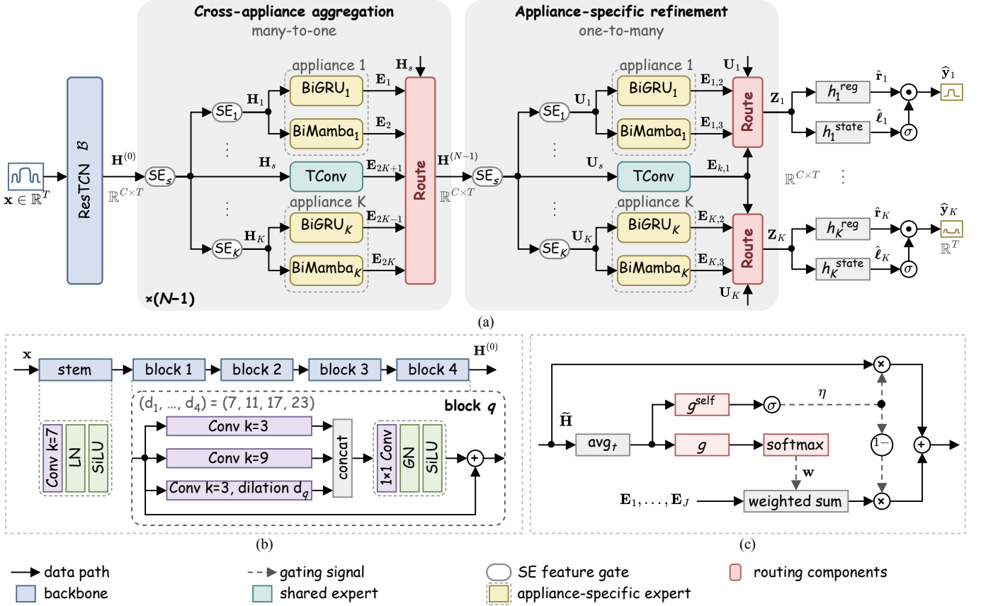
Fig. 1. FLAME architecture. (a) Forward topology from the backbone output \mathbf{H}^{(0)} through the many-to-one aggregation levels and the one-to-many refinement level to the appliance representations \mathbf{Z}_k and their prediction heads; rows k=1 and k=K stand for all K appliances, and line styles and colors are defined in the legend (SE: squeeze-and-excitation). (b) The ResTCN backbone of (3), with the stem and one residual block expanded (LN: layer normalization, GN: group normalization). (c) The routing operator \text{Route}(\cdot) of (4) and (5), used with J=2K+1 in (7) and J=3 in (9).
