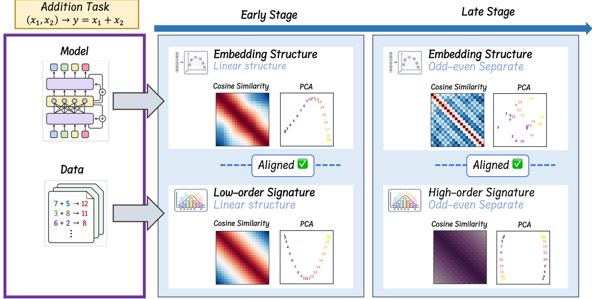
Figure 1: Under small initialization, the embedding geometry evolves progressively during training.
