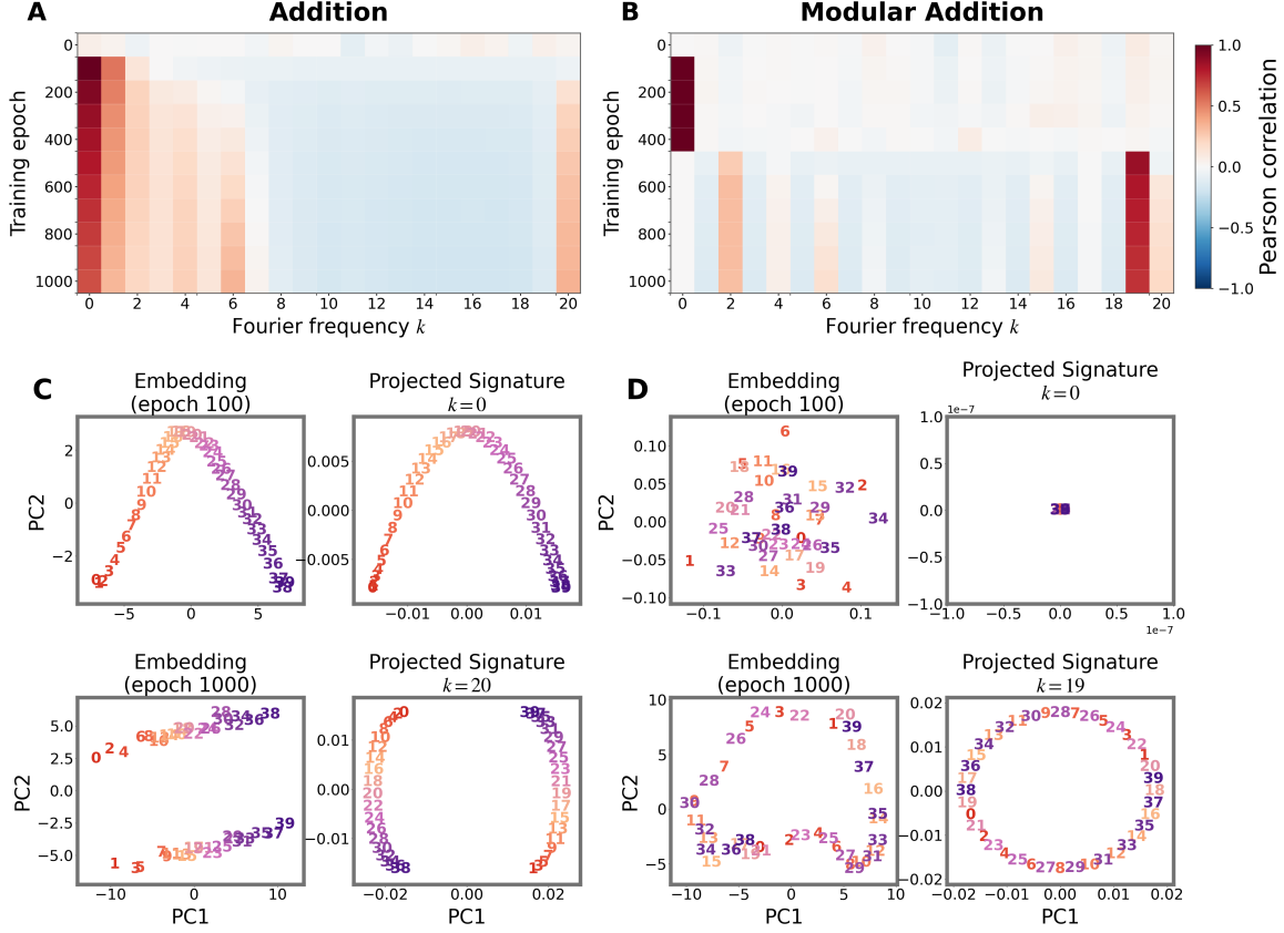
Figure 4: A: Heatmap of \rho_{(1),k}^{(t)} across training epochs t and Fourier frequencies k for the addition task. B: The same correlation heatmap for the modular-addition task. C: PCA projections for the addition task, showing \mathbf{w}_\alpha^E at epochs 100 and 1000 together with \mathbf{h}_{\alpha,k}^{(1)} at frequencies k = 0 and k = 20 , respectively. D: PCA projections for the modular-addition task, showing \mathbf{w}_\alpha^E at epochs 100 and 1000 together with \mathbf{h}_{\alpha,k}^{(1)} at frequencies k = 0 and k = 19 , respectively.
