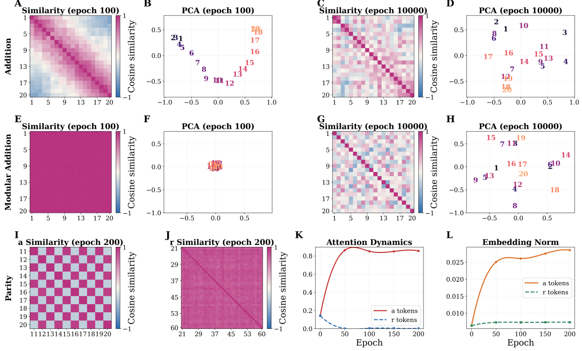
Figure 6: A–H: Embedding cosine-similarity matrices and PCA projections for the addition and modular-addition tasks at early and late training stages. A,B show early-stage addition; C,D show late-stage addition; E,F show early-stage modular addition; G,H show late-stage modular addition. I,J: Embedding cosine-similarity matrices of anchor tokens and noise tokens in the parity task. K: Mean attention dynamics for anchor tokens and noise tokens. L: Embedding norm dynamics for anchor tokens and noise tokens.
