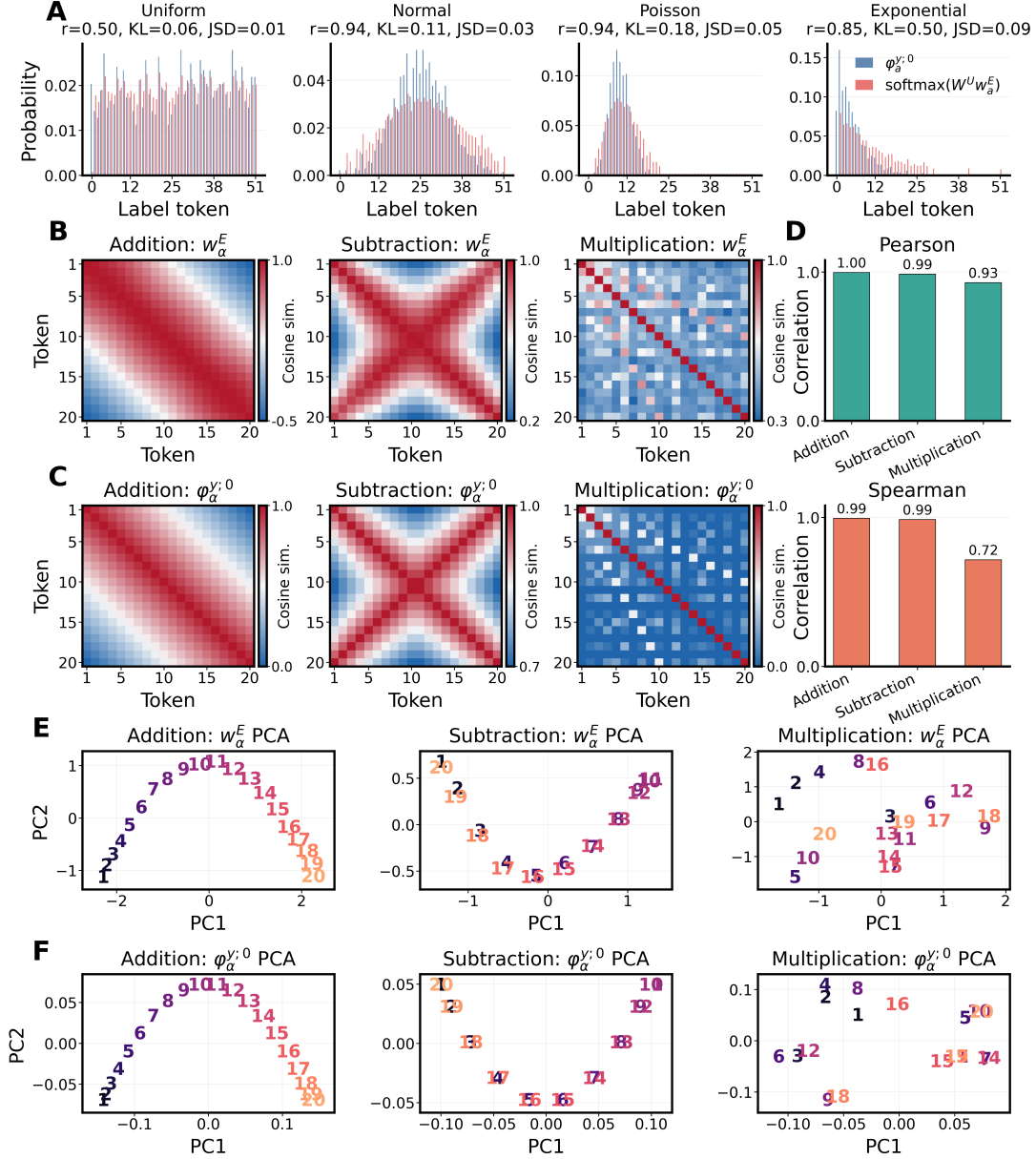
Figure 2: A: Comparison between the \varphi_a^{y;0} and \text{softmax}(\mathbf{W}^U \mathbf{w}_a^E) in Task 1 under four target label distributions: uniform, normal, Poisson, and exponential. Here, r denotes the Pearson correlation coefficient, KL denotes the Kullback–Leibler divergence, and JSD denotes the Jensen–Shannon divergence between the two distributions. B: Heatmap of S^{\text{emb},(t)} for the addition, absolute-subtraction, and multiplication tasks, with t = 100 . C: Heatmap of S^{\text{sig}} for the three arithmetic tasks. D: Pearson and Spearman correlations between the off-diagonal entries of S^{\text{emb},(t)} and S^{\text{sig}} across the three arithmetic tasks, where t = 100 . E: PCA projections of the learned token embeddings for the three arithmetic tasks at epoch 100. F: PCA projections of the corresponding zero-order label signatures for the three arithmetic tasks.
