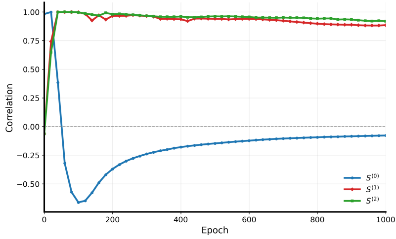
Figure 13: Correlation between the off-diagonal entries of the anchor-token embedding cosine-similarity matrix and the similarity matrices induced by the zeroth-, first-, and second-order signatures, denoted by S^{(0)} , S^{(1)} , and S^{(2)} , respectively, over training epochs. The horizontal dashed line marks zero correlation.
