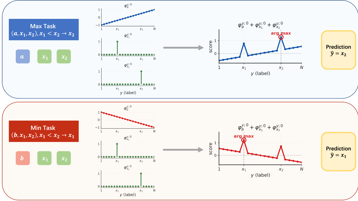
Figure 10: Mechanism of zero-order signature superposition in the min-max task.
