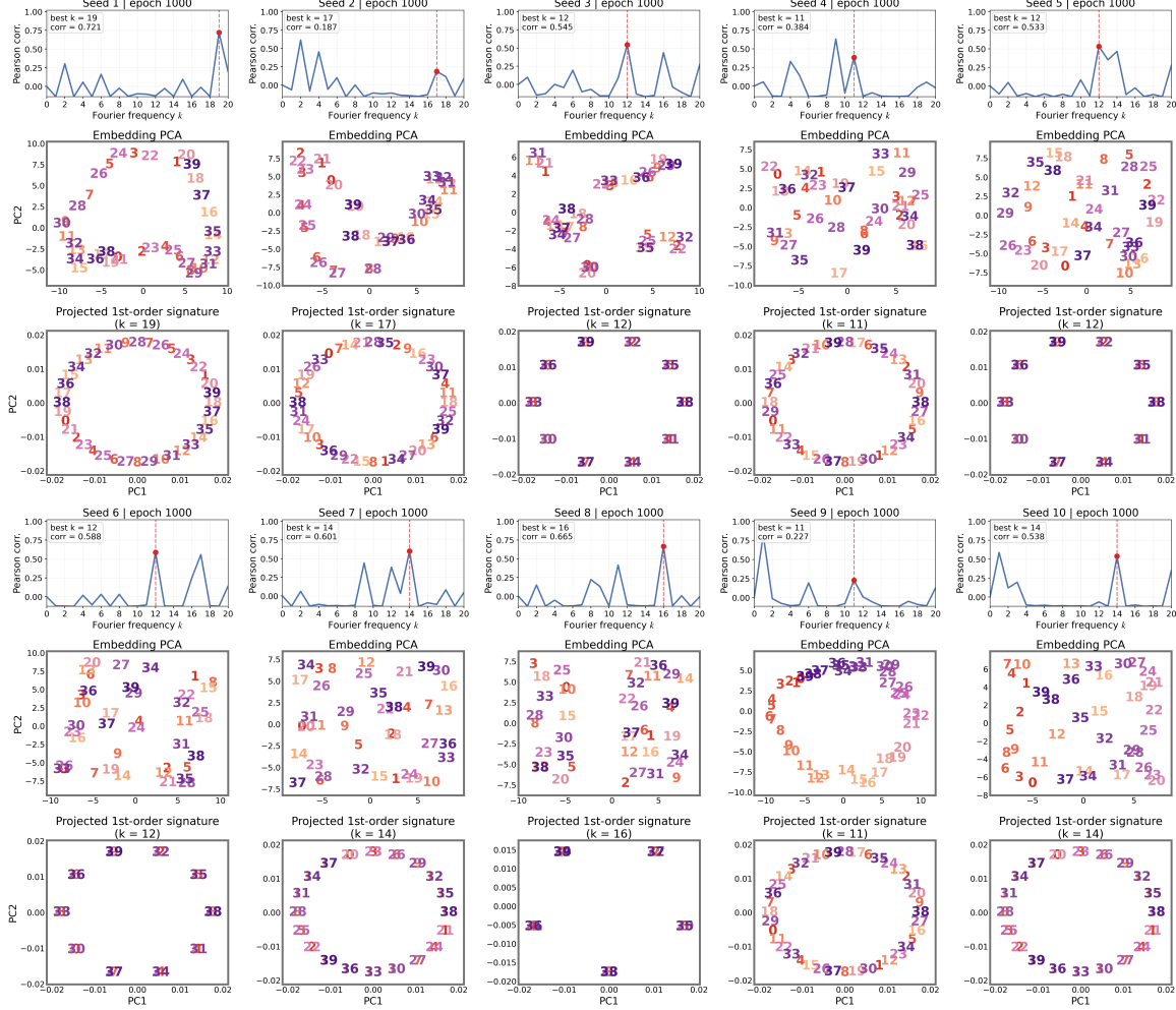
Figure 14: Results for ten random seeds at epoch 1,000. For each seed, the top panel shows the Pearson correlation between the embedding similarity structure and that induced by each Fourier frequency k of the first-order signature, with the red marker and dashed line indicating the frequency of maximum correlation. The middle and bottom panels show the two-dimensional PCA projections of the learned embeddings and the first-order signature component at the selected frequency, respectively. Token indices are displayed directly in the PCA projections.
