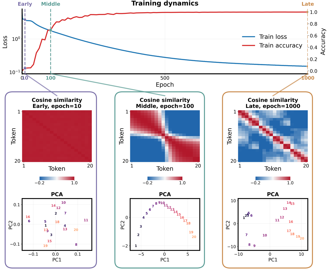
Figure 12: The top panel shows the training loss and accuracy over 1,000 epochs, with dashed vertical lines marking the early, middle, and late checkpoints at epochs 10, 100, and 1,000. The three lower columns show the anchor-token cosine-similarity matrices and their two-dimensional PCA projections at the corresponding checkpoints. Token indices are displayed directly in the PCA projections.
