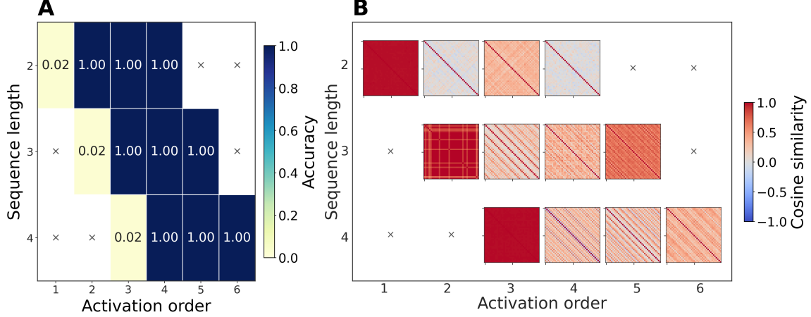
Figure 5: A: Heatmap of the maximum training accuracy achieved for modular-addition tasks with different sequence lengths and activation orders. B: Cosine-similarity matrices of the learned token embeddings for the corresponding task settings with different sequence lengths and activation orders.
