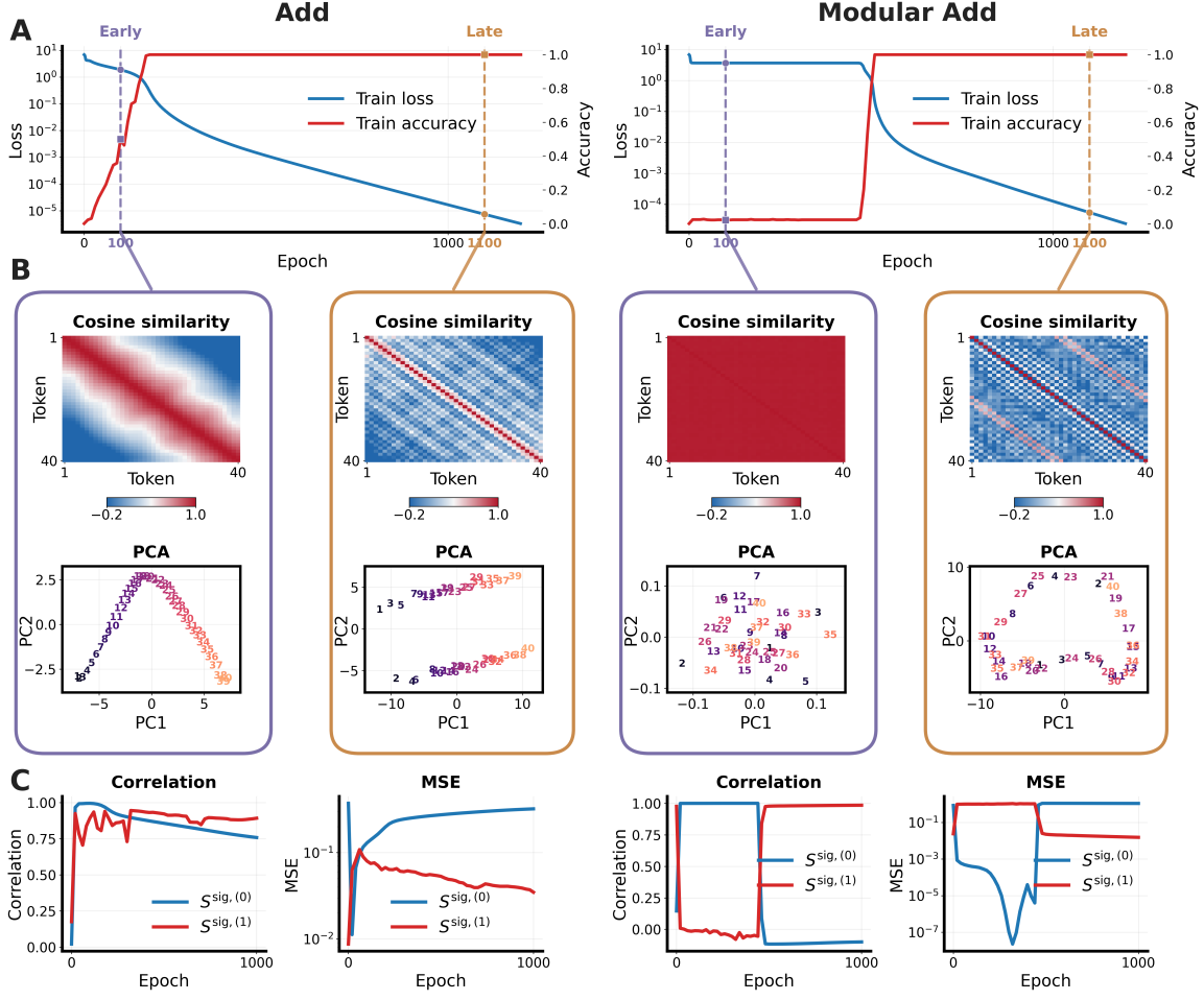
Figure 3: A: Training loss and training accuracy over epochs for the addition task and the modular-addition task. The dashed vertical lines mark the early and late epochs used for visualization. B: Cosine-similarity matrices and PCA projections of the learned token embeddings at the early and late epochs for the addition task and the modular-addition task. C: Temporal evolution of the correlation and MSE between the S^{\text{emb},(t)} and the S^{\text{sig},(0)} , as well as the optimized \tilde{S}^{\text{sig},(1)} , for the addition task and the modular-addition task.
