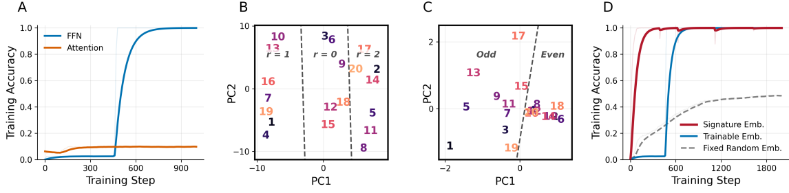
Figure 8: A: Training accuracy of the FFN model and the attention-only model. B: PCA projection of the final FFN token embeddings. C: PCA projection of the final attention-only token embeddings. D: Training accuracy of the FFN model with fixed first-order signature embeddings, trainable embeddings, and fixed random embeddings.
