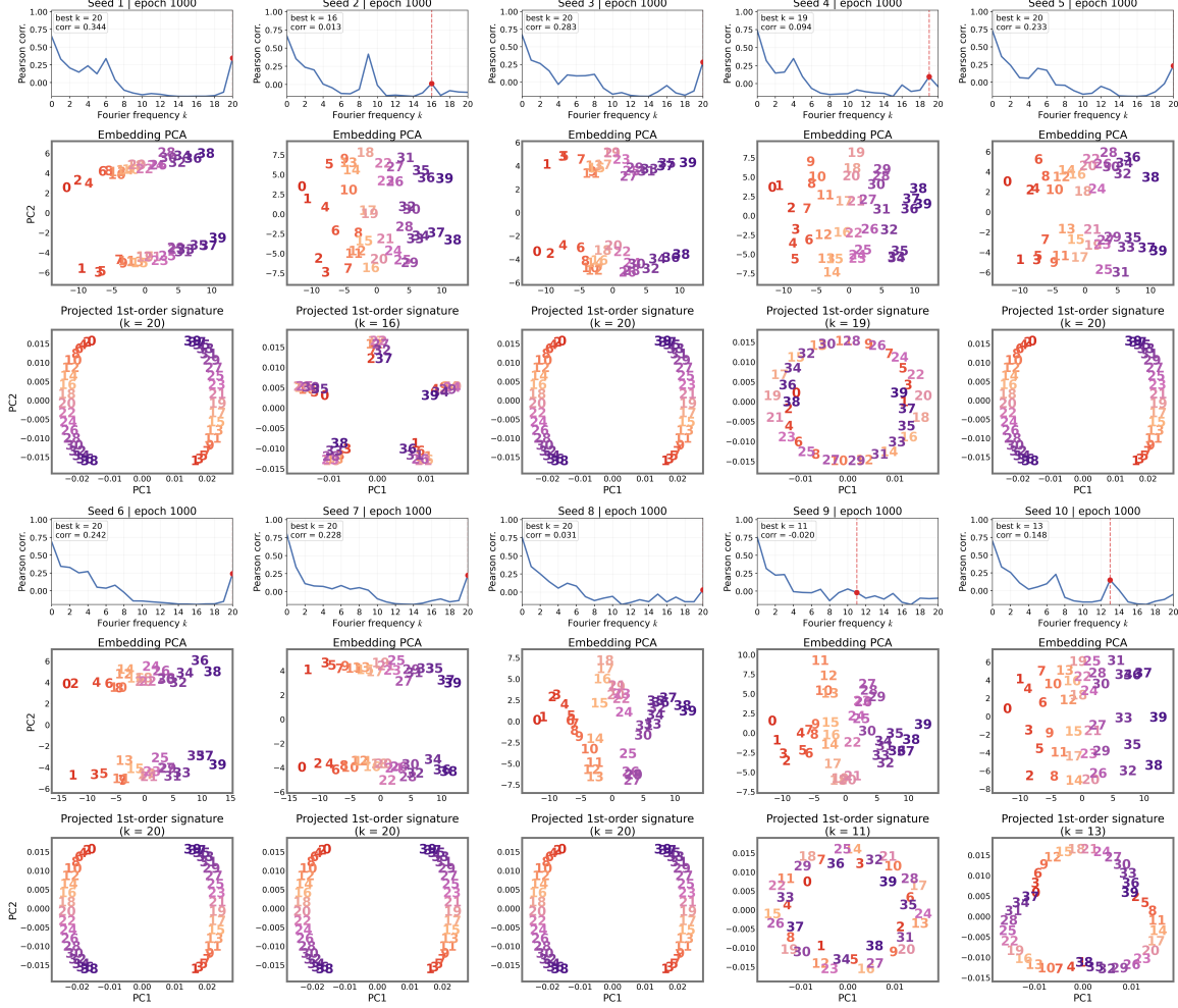
Figure 15: Results for ten random seeds at epoch 1,000. For each seed, the top panel shows the Pearson correlation between the embedding similarity structure and that induced by each Fourier frequency k of the first-order signature, with the red marker and dashed line indicating the frequency of maximum correlation. The middle and bottom panels show the two-dimensional PCA projections of the learned embeddings and the first-order signature component at the selected frequency, respectively. Token indices are displayed directly in the PCA projections.
