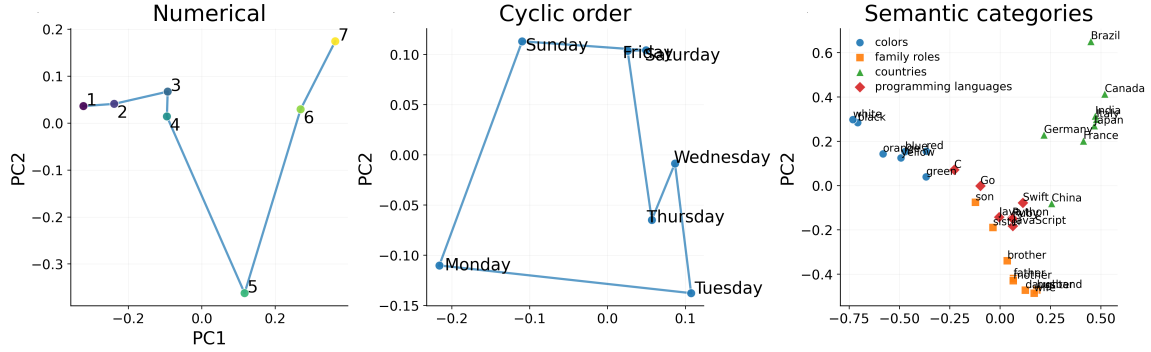
Figure 11: A: PCA projection of the signatures of numerical tokens, connected according to their numerical order. B: PCA projection of the signatures of weekdays, connected according to their cyclic order. C: Joint PCA projection of the signatures of tokens from different semantic categories, including colors, family roles, countries, and programming languages.
