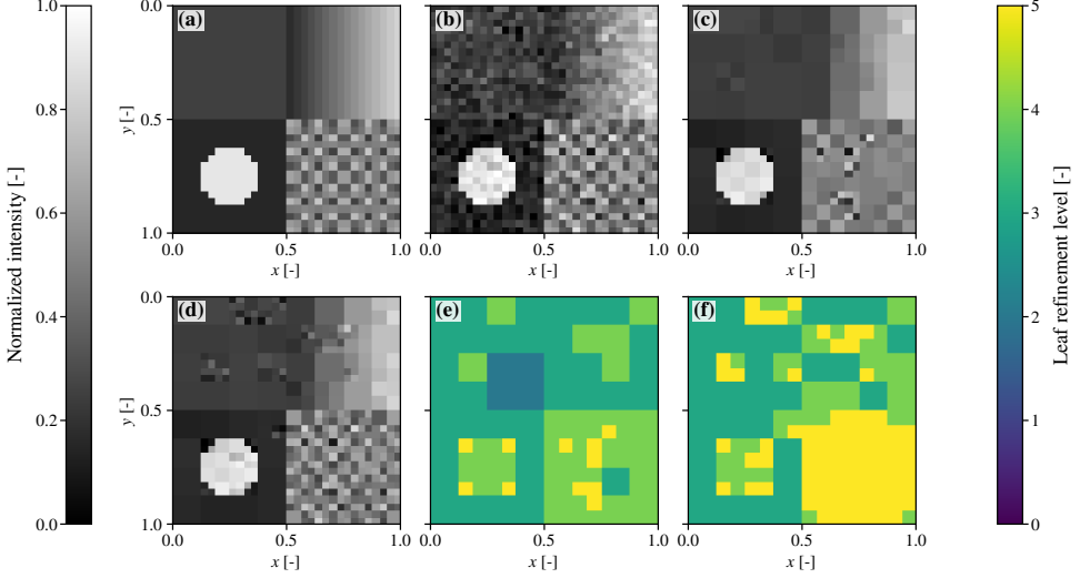
FIG. 1. Representative spatial outcome for the four-region holdout case: (a) clean image; (b) noisy input; (c) deterministic-AMDI reconstruction; (d) Learned-AMDI reconstruction; (e) final deterministic-AMDI refinement levels; and (f) final learned refinement levels. This figure illustrates the terminal allocations; sequential contribution is assessed separately by the decision-1-only control.
