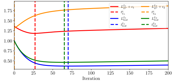
Figure 2: Curves L_{\mathcal{D}}^{L_p} and L_{test}^{L_p} for Gaussian distribution ( m = 256, n = 512 ). We check that L_{test}^{L_p} is below L_{\mathcal{D}}^{L_p} ( p = 1, 2 ), and t_{L_1}^* closer than t_{L_2}^* to t_{test}^{L_p} for p = 1 and 2.
