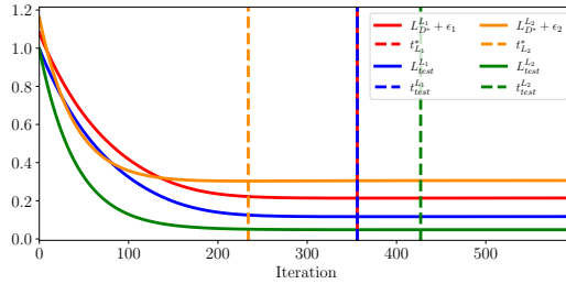
Figure 6: Curves L_{\mathcal{D}^*}^{Lp} + \epsilon_p and L_{test}^{Lp} for classification 3-5. We check that L_{test}^{Lp} is below L_{\mathcal{D}^*}^{Lp} + \epsilon_p ( p = 1, 2 ), and t_{L_1}^* closer than t_{L_2}^* to t_{test}^{Lp} for p = 1 and p = 2 .
