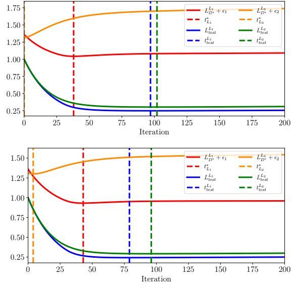
Figure 10: Uniform distribution. Top: m = 512, n = 512 ( \lambda_1 \equiv \lambda_\alpha = 2413, \lambda_2 = 679 ). Bottom: m = 256, n = 512 ( \lambda_1 \equiv \lambda_\alpha = 2291, \lambda_2 = 486 ).
