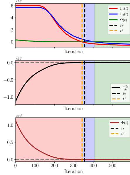
Figure 5: Top: sign-invariant subintervals \mathcal{T}_1 = [0, 343) , \mathcal{T}_2 = [343, 407) , \mathcal{T}_3 = [407, 600) with curves \Gamma_1, \Gamma_2, \Omega . Middle: curve dL_{\mathcal{D}}^*/dt . Bottom: curve \Phi(t) . We have t^+ = 342 \approx \tau_1 = 343 \leq t^* = 357 (case 2 of Proposition 7).
