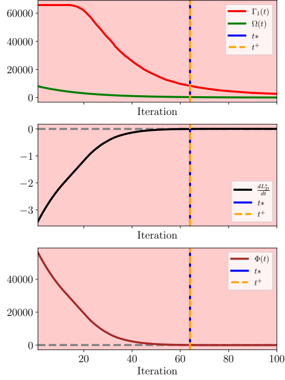
Figure 3: Top: the sign-invariant subinterval \mathcal{T}_1 = [0, 100) with curves \Gamma_1, \Omega . Middle: curve dL_{\mathcal{D}}^*/dt . Bottom: curve \Phi(t) . We have t^+ = t^* = 64 < \tau_1 (case 1).
