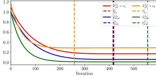
Figure 8: Curves L_{\mathcal{D}}^{L_p} + \epsilon_p and L_{\text{test}}^{L_p} for classification 0-1. We check that L_{\text{test}}^{L_p} is below L_{\mathcal{D}}^{L_p} + \epsilon_p ( p = 1, 2 ), and t_{L_1}^* closer than t_{L_2}^* to t_{\text{test}}^{L_p} for p = 1 and p = 2 .
