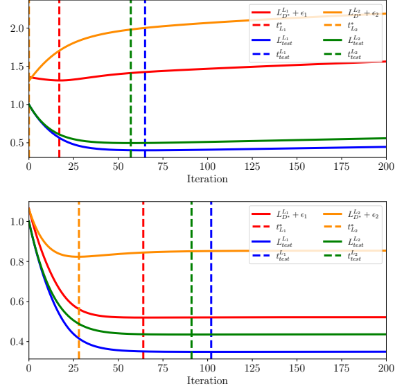
Figure 9: Gaussian distribution. Top: m = 512, n = 512 ( \lambda_1 \equiv \lambda_\alpha = 2291, \lambda_2 = 486 ). Bottom: m = 256, n = 16384 ( \lambda_1 \equiv \lambda_\alpha = 8.23 \cdot 10^4, \lambda_2 = 2.05 \cdot 10^4 ).
