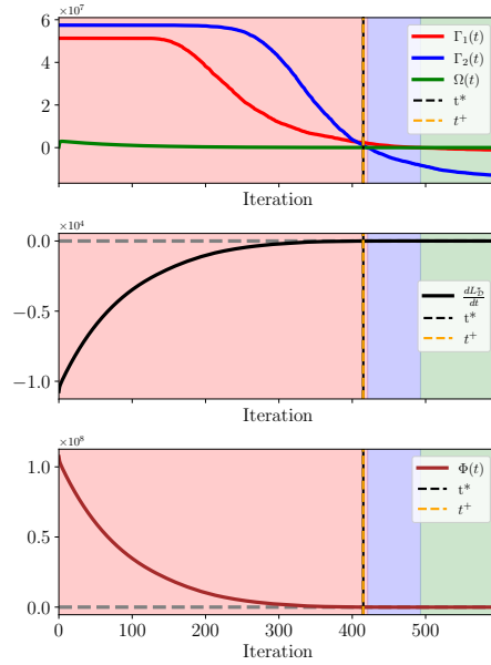
Figure 7: Top: sign-invariant subintervals \mathcal{T}_1 = [0, 421) , \mathcal{T}_2 = [421, 493) , \mathcal{T}_3 = [493, 600) with curves \Gamma_1, \Gamma_2, \Omega . Middle: curve dL_{\mathcal{D}}^*/dt . Bottom: curve \Phi(t) . We have t^+ = t^* = 415 < \tau_1 = 421 (case 1).
