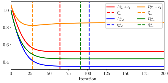
Figure 4: Curves L_{\mathcal{D}}^{Lp} and L_{test}^{Lp} for Gaussian distribution ( m = 256 , n = 16384 ). We check that L_{test}^{Lp} is below L_{\mathcal{D}}^{Lp} ( p = 1, 2 ), and t_{L1}^* closer than t_{L2}^* to t_{test}^{Lp} for p = 1 and 2.
