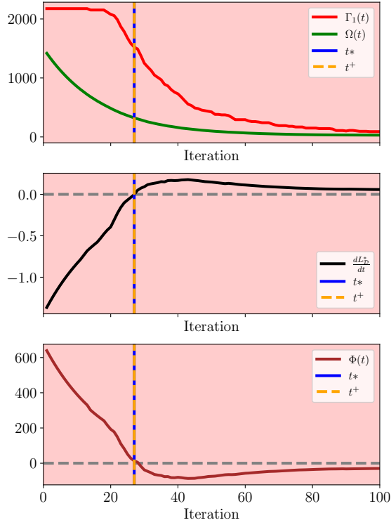
Figure 1: Top: the sign-invariant subinterval \mathcal{T}_1 = [0, 100) with curves \Gamma_1, \Omega . Middle: curve dL_{\mathcal{D}}^*/dt . Bottom: curve \Phi(t) . We have t^+ = t^* = 27 < \tau_1 = 100 (case 1 of Proposition 7).
