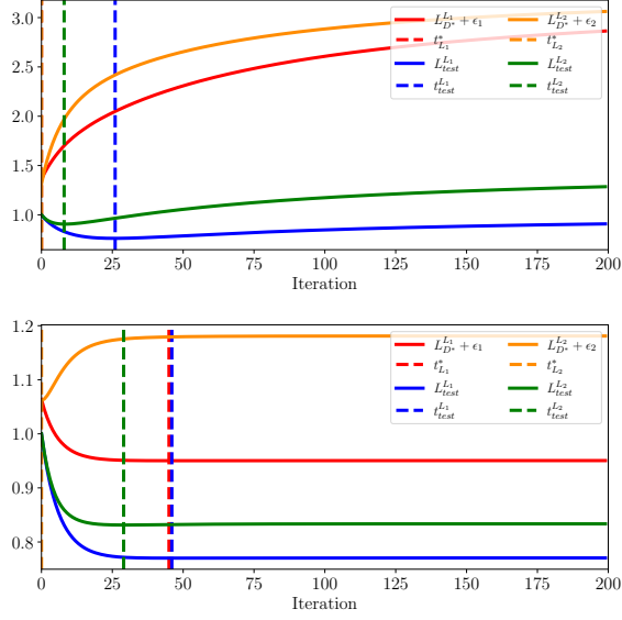
Figure 11: Pareto distribution. Top: m = 256 , n = 512 . ( \lambda_1 \equiv \lambda_\alpha = 5 \cdot 10^5 , \lambda_2 = 1 \cdot 10^5 ). Bottom: m = 256 , n = 16384 . ( \lambda_1 \equiv \lambda_\alpha = 17 \cdot 10^6 , \lambda_2 = 3 \cdot 10^6 ).
