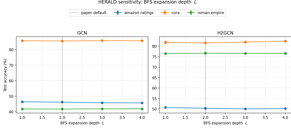
Fig. D3 Accuracy vs. BFS expansion depth L \in [1, 4] . BFS depth is the most structurally impactful parameter: increasing L from 1 to 4 on Amazon-ratings reduces the condensed node count from 21,755 to 17,048 (SR from 88.7% to 69.4%) because deeper trees are more expensive per root, admitting fewer roots within the budget. The accuracy swing of 0.71% on Amazon-ratings GCN reflects this structural difference rather than the scoring criterion per se.
