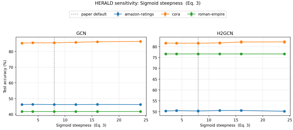
Fig. D2 Accuracy vs. sigmoid steepness c \in [2, 24] . The largest swing (1.07% GCN on Cora) occurs because a higher steepness pushes Cora’s very low h even further below the midpoint, slightly raising the prototype weight and shifting which nodes are ranked highest. Amazon-ratings and Roman-empire are unaffected.
