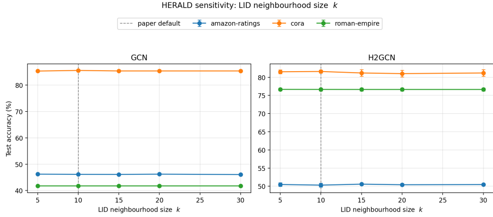
Fig. D4 Accuracy vs. LID neighbourhood size k \in [5, 30] . All curves are nearly flat; the largest swing (0.59% H2GCN on Cora) is within the standard deviation of the baseline. LID estimates stabilise quickly with neighbourhood size, and the relative ranking of nodes by LID score is robust even at small k .
