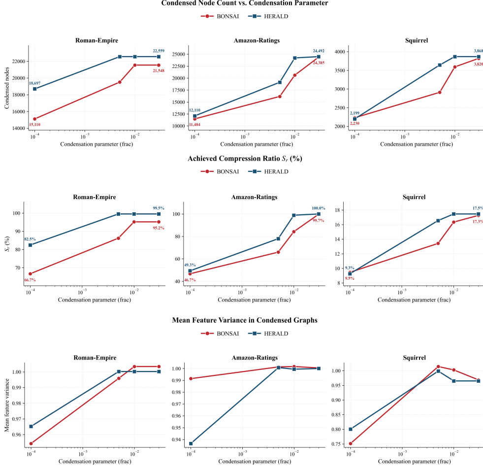
Fig. E5 Structural comparison of BONSAI and HERALD condensed graphs across three datasets and four compression fractions r \in \{10^{-4}, 5 \times 10^{-3}, 10^{-2}, 3 \times 10^{-2}\} . Top: condensed node count |V_c| . HERALD consistently selects more nodes than BONSAI at the same budget, because its Fisher×density feature selection reduces the per-node storage cost f_v , leaving more of the budget for nodes. Middle: achieved storage ratio SR(\%) = \mathcal{C}(G_c)/\mathcal{C}(G) \times 100 . HERALD reaches saturation earlier than BONSAI on Roman-empire and Amazon-ratings, reflecting its higher node-count efficiency. On Squirrel, both condensers saturate near SR \approx 17\% because edge storage dominates the budget. Bottom: normalised mean feature variance \hat{\sigma}^2 (Eq. (E2)). HERALD preserves equal or greater feature diversity at every budget point; the gap is largest at r = 10^{-4} on Squirrel (+0.05 over BONSAI), confirming that the LID diversity term prevents the condensed set from collapsing onto a narrow feature cluster.
