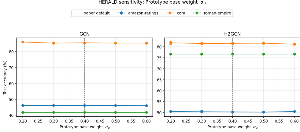
Fig. D1 Accuracy vs. prototype base weight \alpha_0 \in [0.2, 0.6] . All three datasets are essentially flat across the sweep, with swings \leq 0.66\% on Cora and \leq 0.29\% on Amazon-ratings. Roman-empire is unaffected (SR \approx 99.5\% , all variants produce the same condensed graph).
