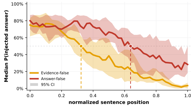
Figure 10: Resisted traces (mirror analysis). Transplant curves for the 40 silent traces that did not take the injected option, transplanted onto the prompt containing the cue. Each curve starts at the cued rate and falls as more of the resisting trace is prefixed. The dot marks x_{50} , the crossing of 50%, as reported in Section 5.2.
