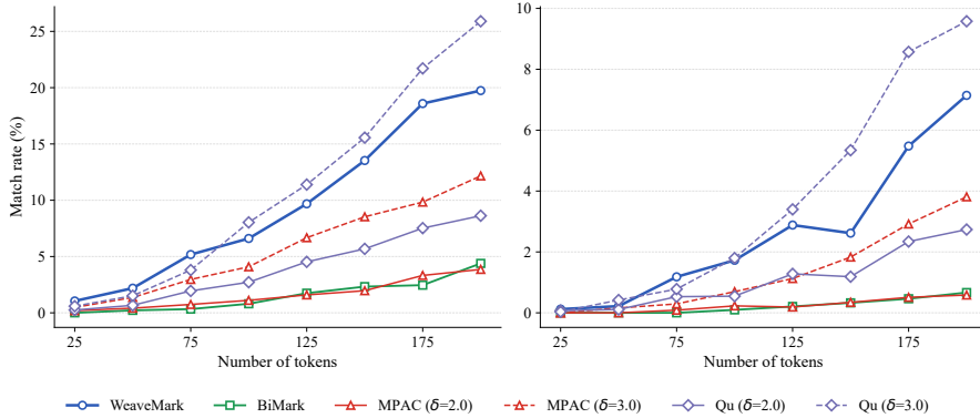
Figure 11: Robustness to stronger synonym substitution attacks with \rho = 0.3 .
