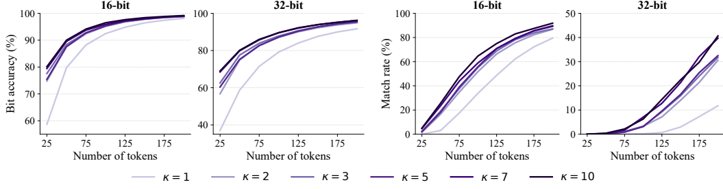
Figure 2: Effect of the number of bits embedded in each token, \kappa , in payload spreading. Increasing \kappa spreads each bit over more token positions, improving both bit accuracy and match rate.
