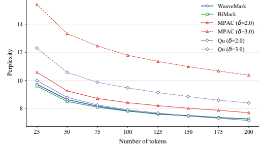
Figure 9: Mean PPL results (16-bit).
