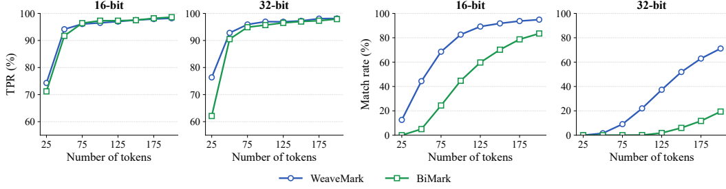
Figure 7: Zero-bit detection in the multi-bit setting at FPR=1%. With \ell = 10 and \ell_z = 2 , WEAVEMARK maintains its multi-bit match-rate advantage while achieving strong zero-bit TPR.
