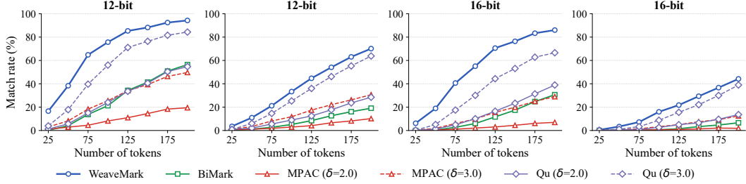
Figure 6: Robustness to synonym substitution attacks. Within each message-length group, the left and right panels use substitution ratios \rho = 0.1 and \rho = 0.2 , respectively.
