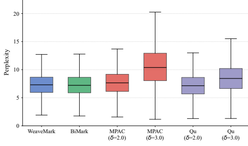
Figure 8: PPL distribution at 200 tokens (16-bit).
