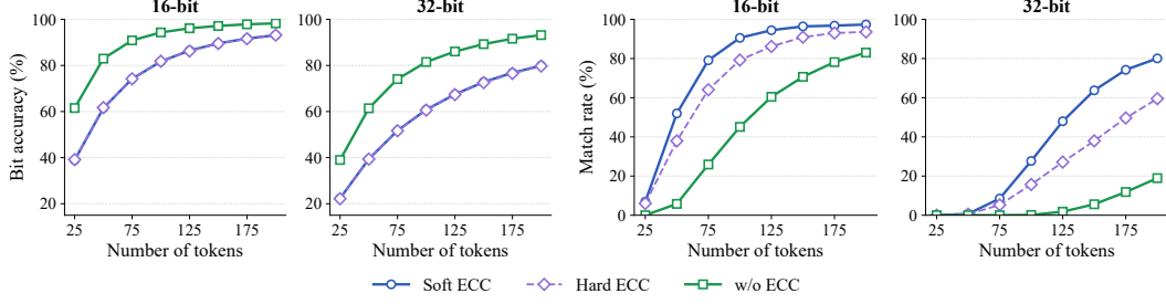
Figure 4: Effect of soft-decision ECC with one-bit-per-token embedding. Soft-decision decoding uses vote margins as reliability information, improving match rate over hard ECC and no ECC.
