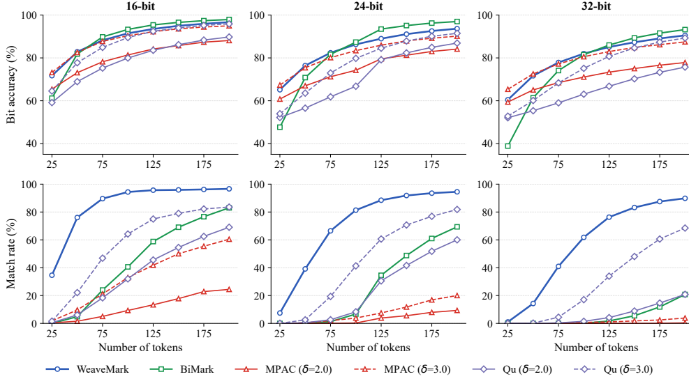
Figure 5: Clean-text message extraction accuracy. WEAVEMARK improves match rate across token lengths, enabling reliable 32-bit payload recovery beyond the range of prior methods.
