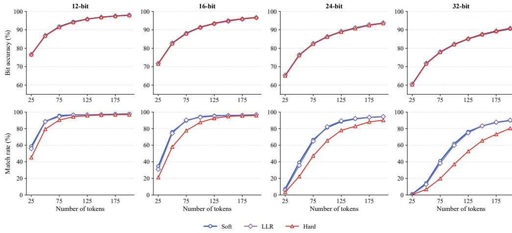
Figure 10: Comparison of hard, soft, and LLR voting across message lengths.
