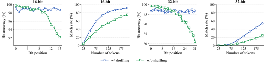
Figure 3: Effect of layer shuffling in payload spreading. Bit-position accuracy is measured at 200 tokens. Layer shuffling balances layer reliability across bit positions, improving match rate.
