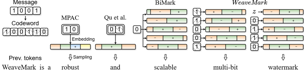
Figure 1: Conceptual comparison of representative multi-bit LLM watermarking methods. Each column represents a distinct scheme. Colors denote vocabulary partitions, +/− signs indicate reweighting directions, and hatched bits denote ECC codeword bits. WEAVEMARK weaves multiple codeword bits into each token across layers and uses soft-decision ECC decoding.
