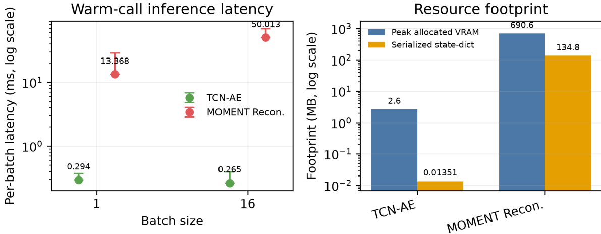
Figure 2: Standardized local resource audit on one RTX 4090. The left panel reports same-process warm-call per-batch p50 latency and p50–p95 ranges over 30 repetitions after 10 warm-ups. The right panel reports peak allocated VRAM and serialized state-dictionary size. Preprocessing and model loading are excluded.
