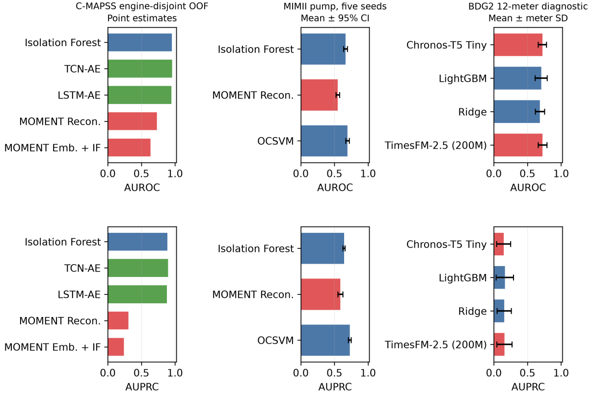
Figure 1: Protocol-specific AUROC and AUPRC; values should not be compared across datasets. Blue denotes classical or fitted baselines, green compact neural models, and red TSFMs. C-MAPSS reports engine-count-weighted means from engine-disjoint folds. MIMII reports five-seed means with t -based 95% confidence-interval half-widths. BDG2 reports meter-macro means with across-meter standard deviations after averaging injection seeds within each meter; these values measure synthetic perturbation sensitivity.
